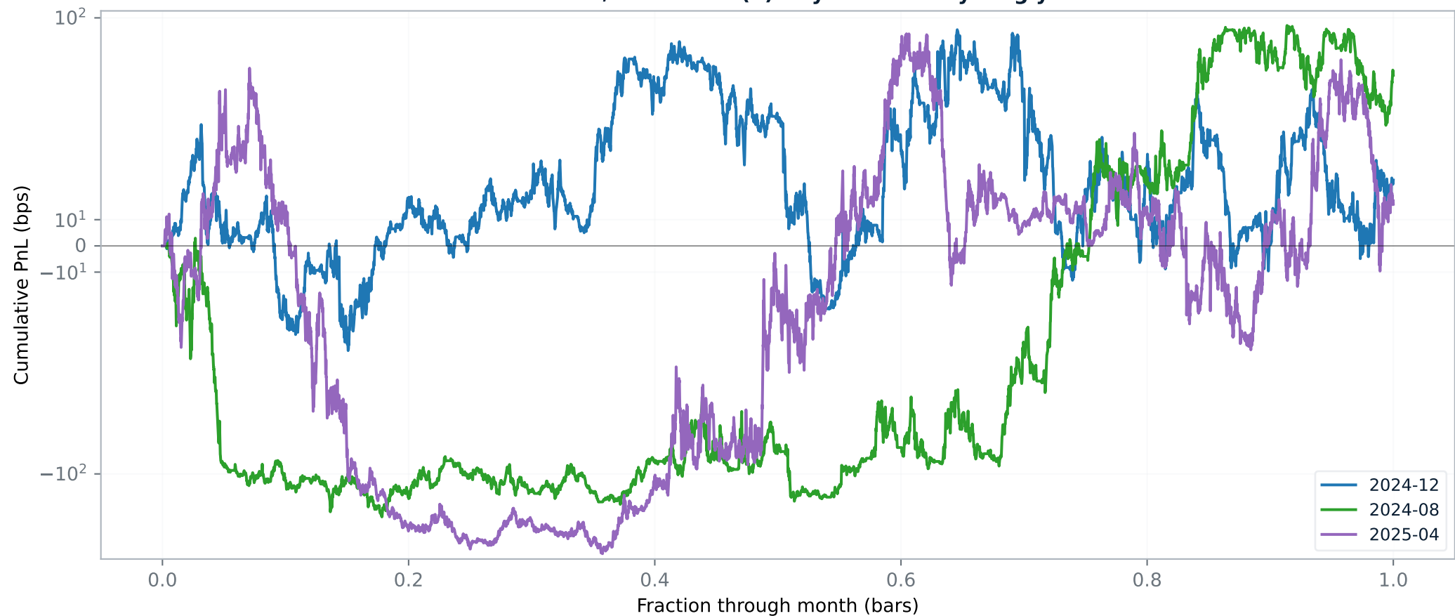
GBPUSD/EURUSD — (1) Buy & Hold — symlog y
