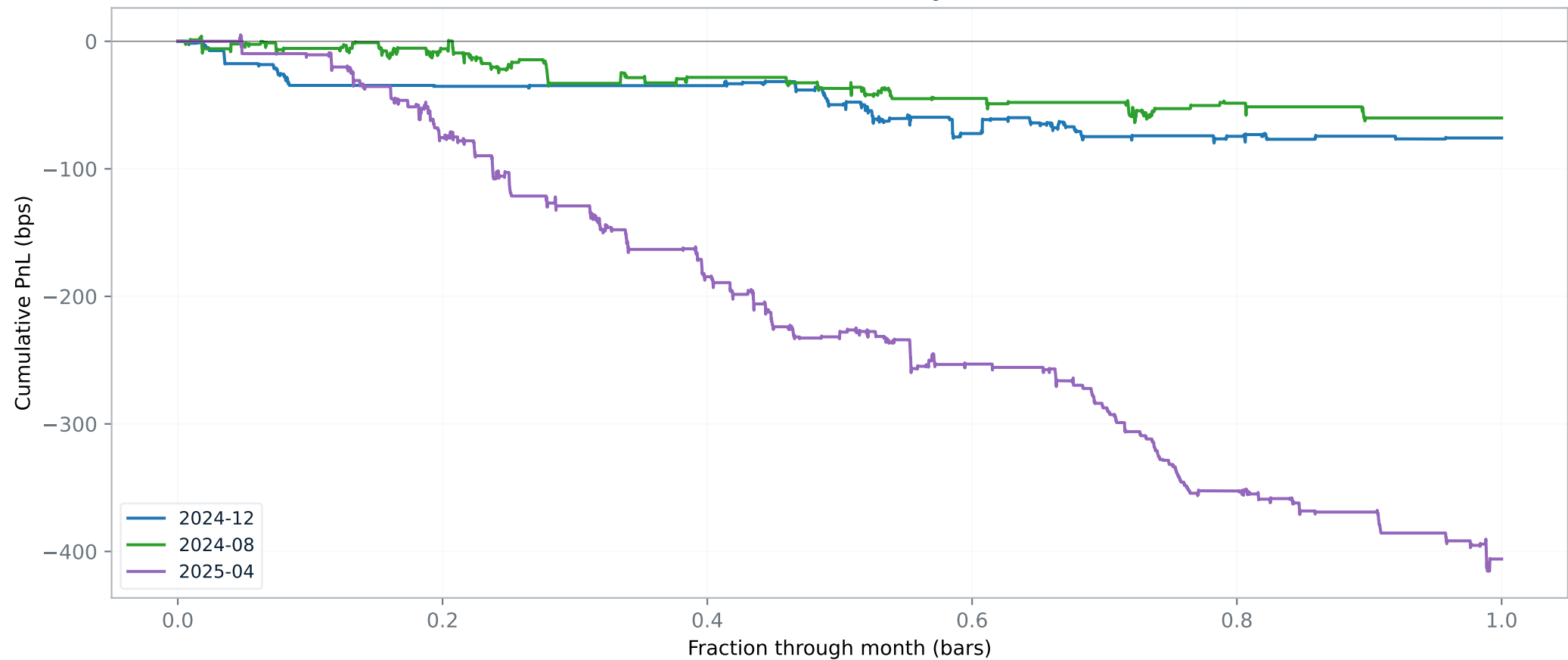
GBPUSD/EURUSD — (4) MS-AR (dynamic threshold)
