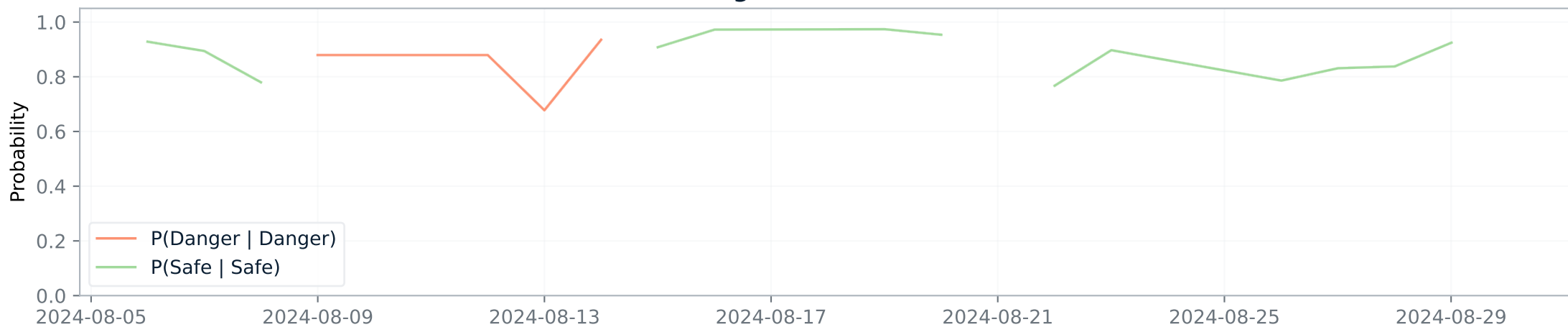
Regime Persistence
