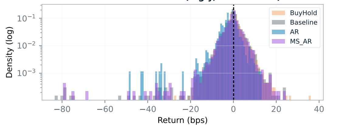
Return Distribution (log y, tails visible)
