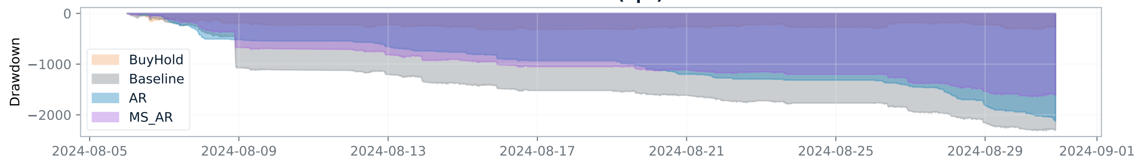
Drawdown (bps)
