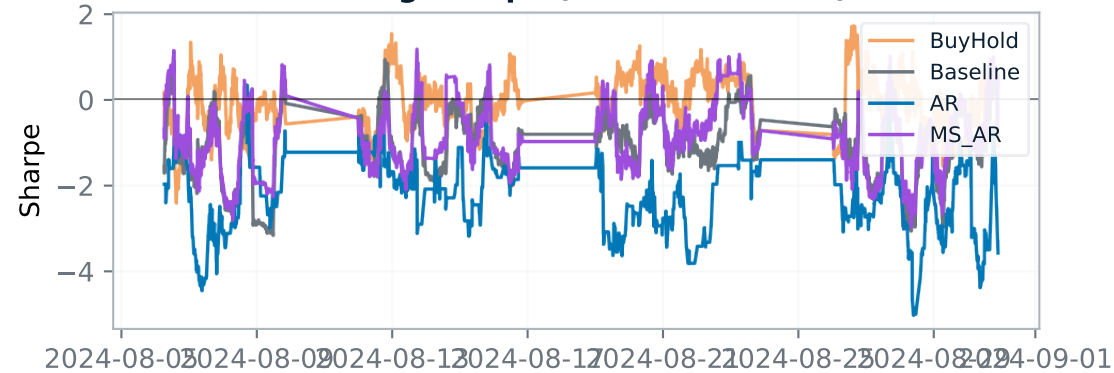
Rolling Sharpe (200-bar window)
