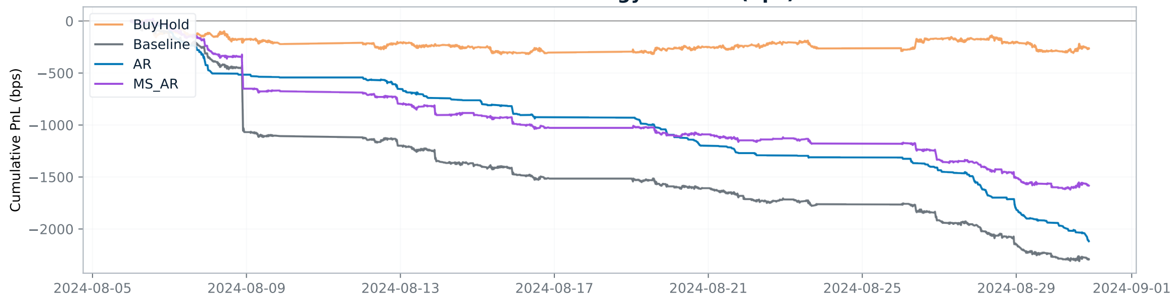
Cumulative Strategy Returns (bps)
