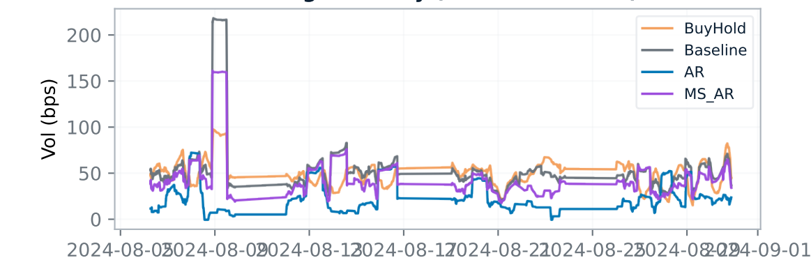
Rolling Volatility (200-bar window)
