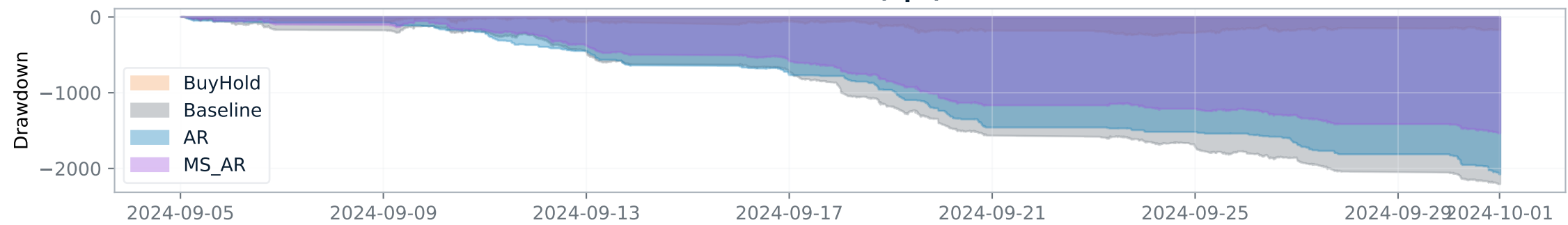
Drawdown (bps)
