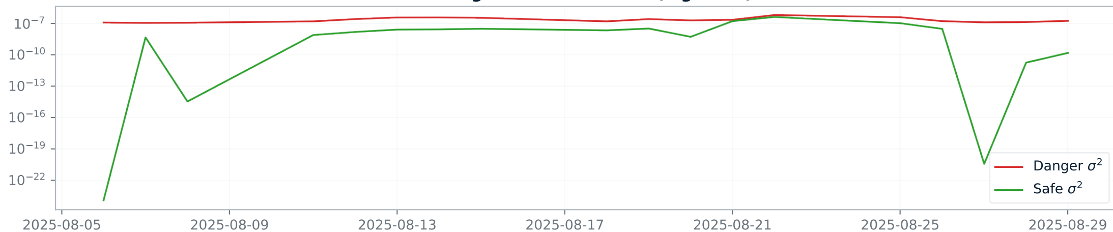
Rolling Markov Variances (log scale)
