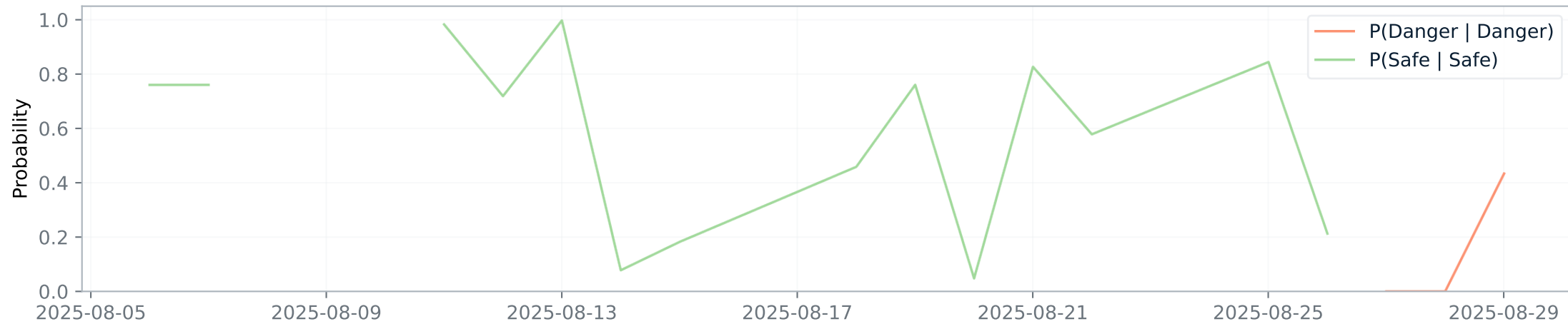
Regime Persistence
