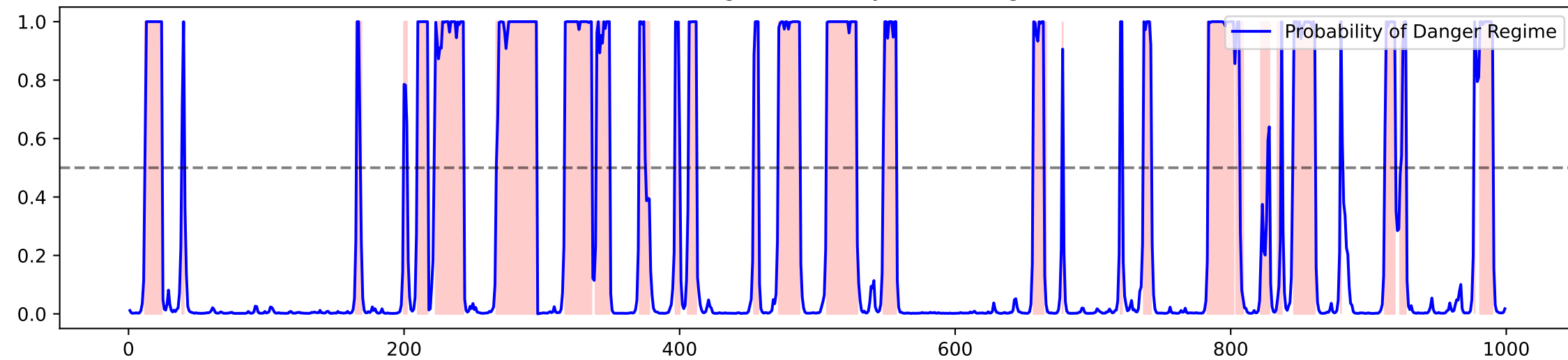
Model Predicted Danger Probability vs True Regimes (Red)
