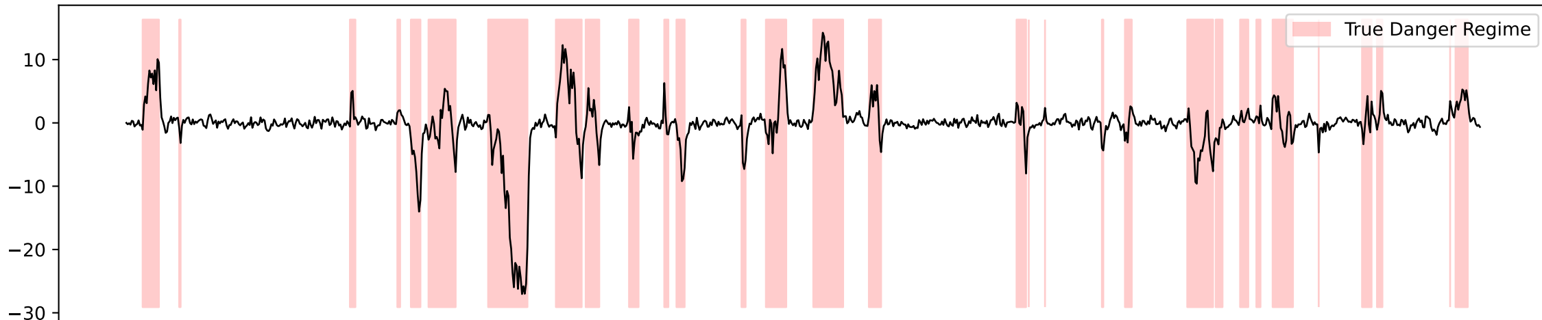
Simulated Pairs Spread (True Regimes)
