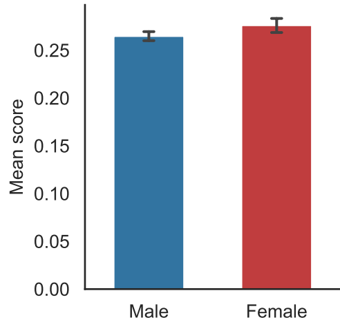
Sentiment
