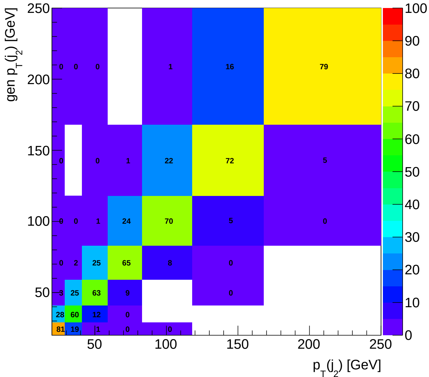
Sherpa Resp. Matrix for 2nd jet p_T ( N_{\text{jets}} \geq 2 )
