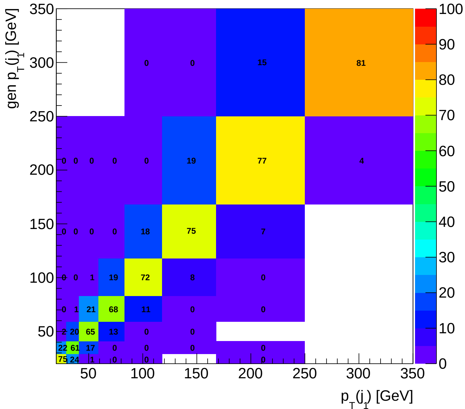
aMC@NLO+Pythia8 Resp. Matrix for 1st jet p_T ( N_{\text{jets}} \geq 1 )
