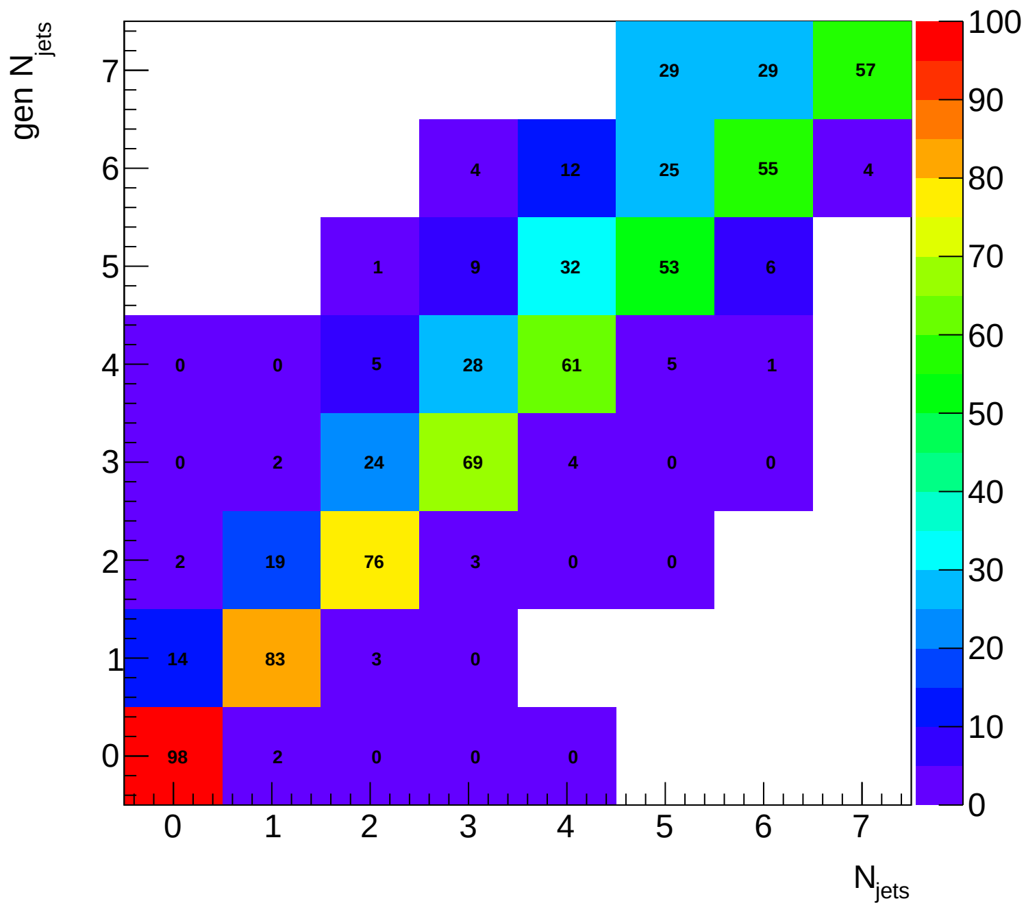
aMC@NLO+Pythia8 Resp. Matrix for Jet Multiplicity (excl.)
