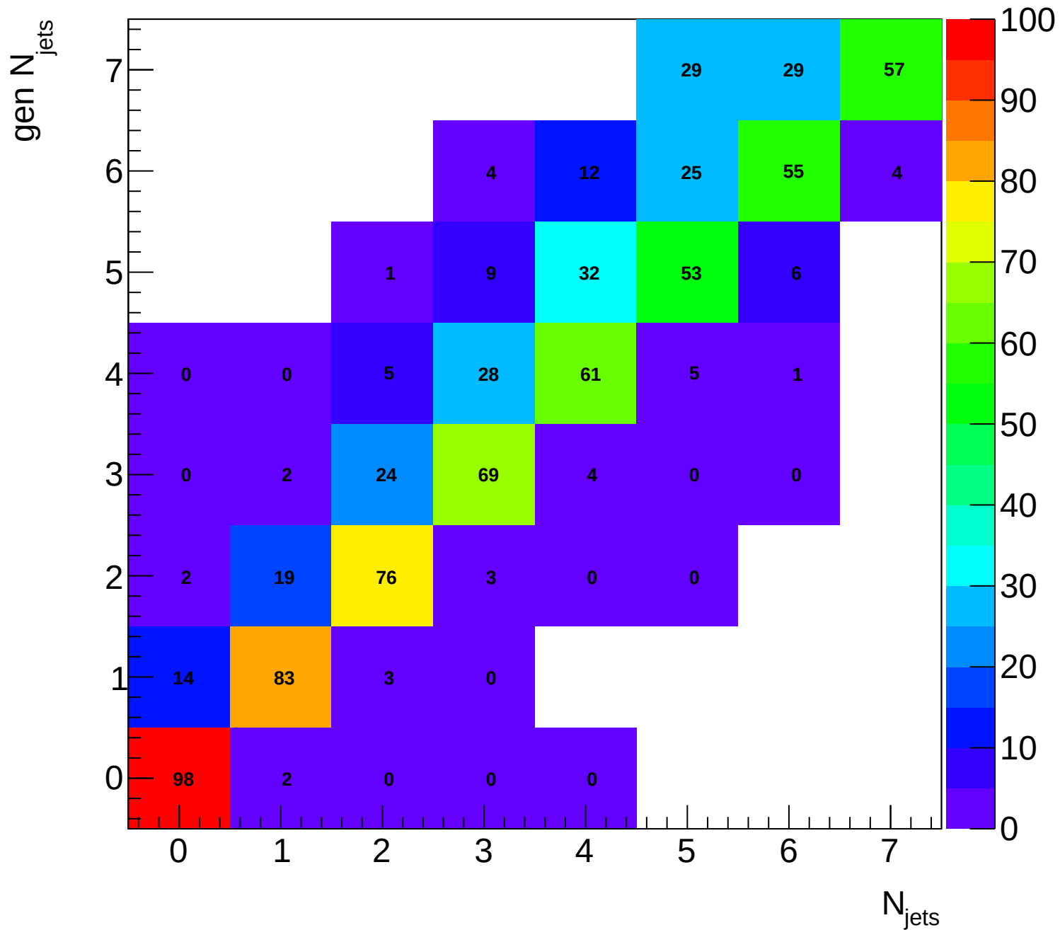
Sherpa Resp. Matrix for Jet Multiplicity (excl.)
