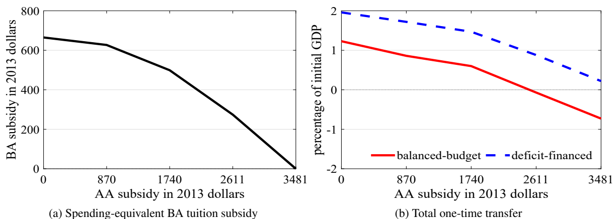
Figure D5: AA and BA subsidy expansion: BA subsidy and total welfare change
