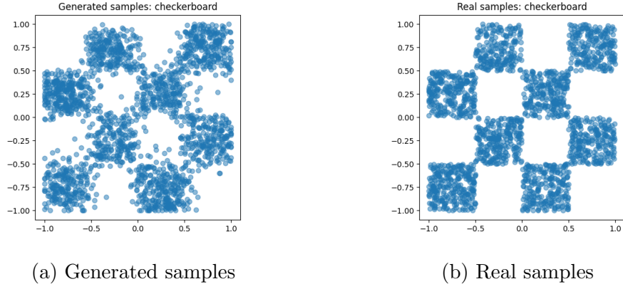
Figure 6: Comparison between generated and real samples for the checkerboard
