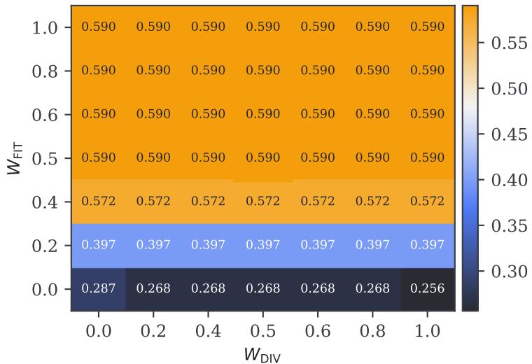
Genre-jump rate
