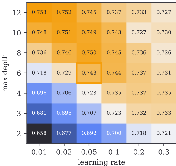
Test AUC vs depth \times lr
