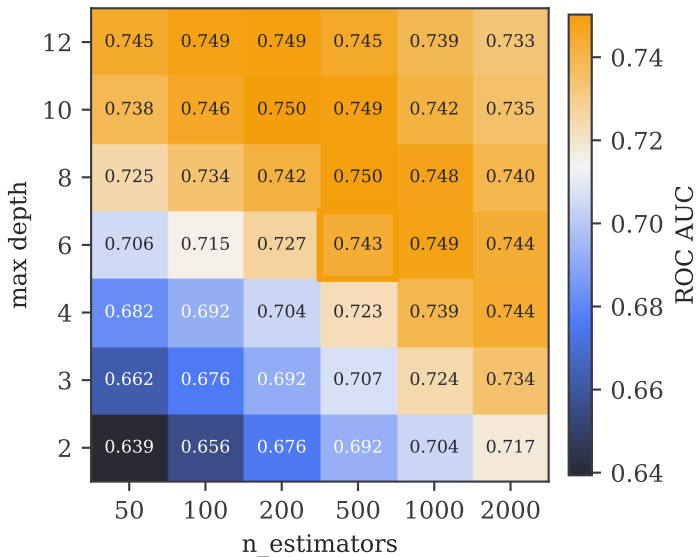
Test AUC vs depth \times n_estimators
