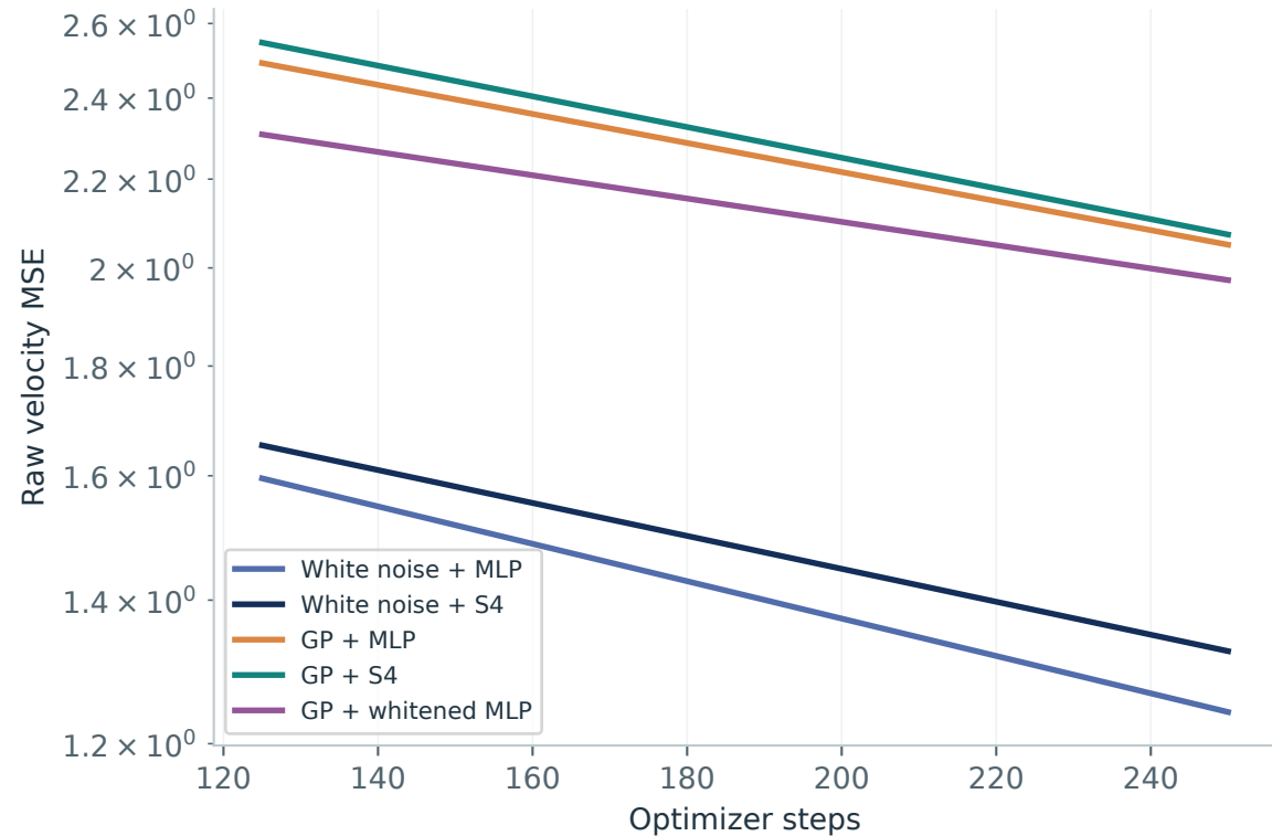
Validation error in observation coordinates
