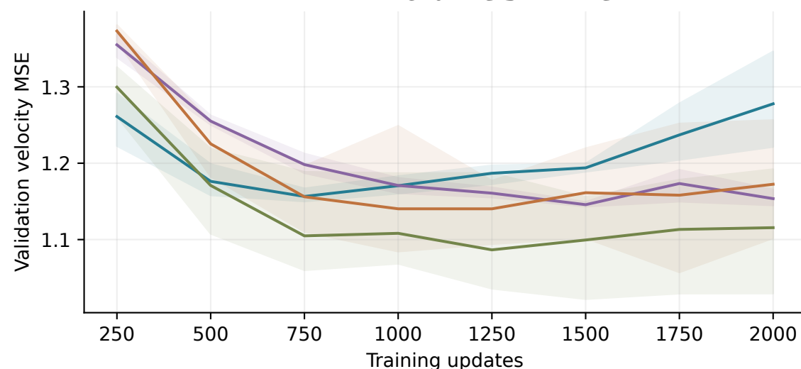
Exchange · 8 channels · white
