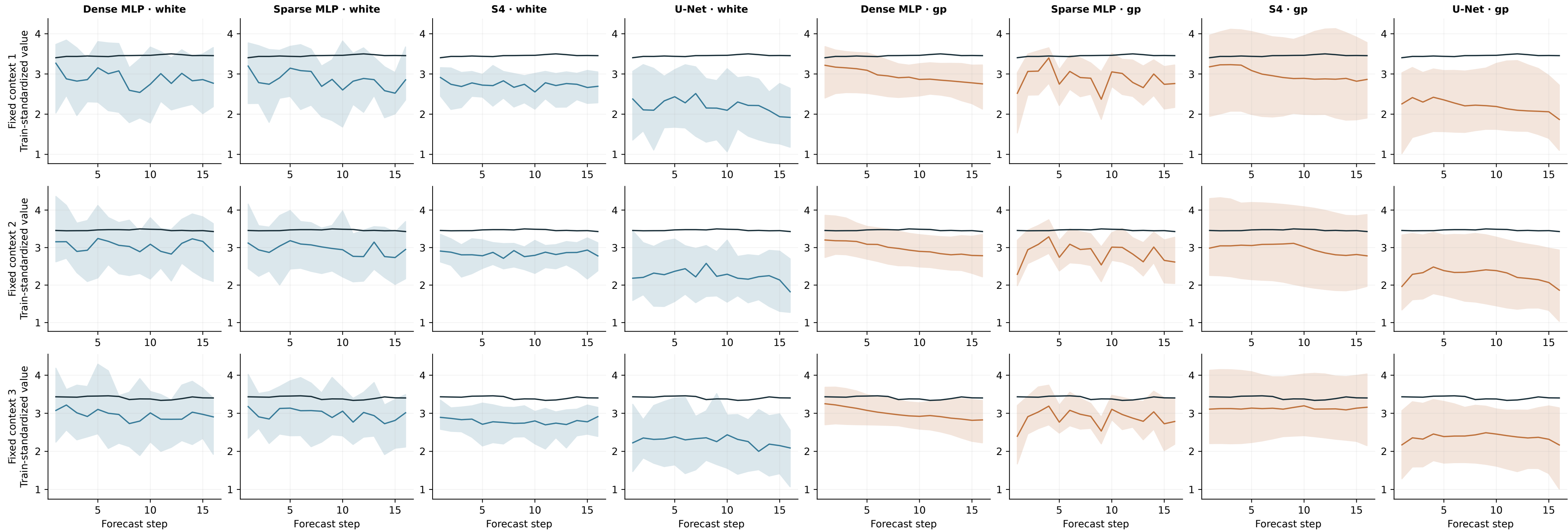
Exchange · 8 channels · channel_7 · first three selected contexts, seed 31 Black: observed future; color: median and marginal 90% band; shared row axes
