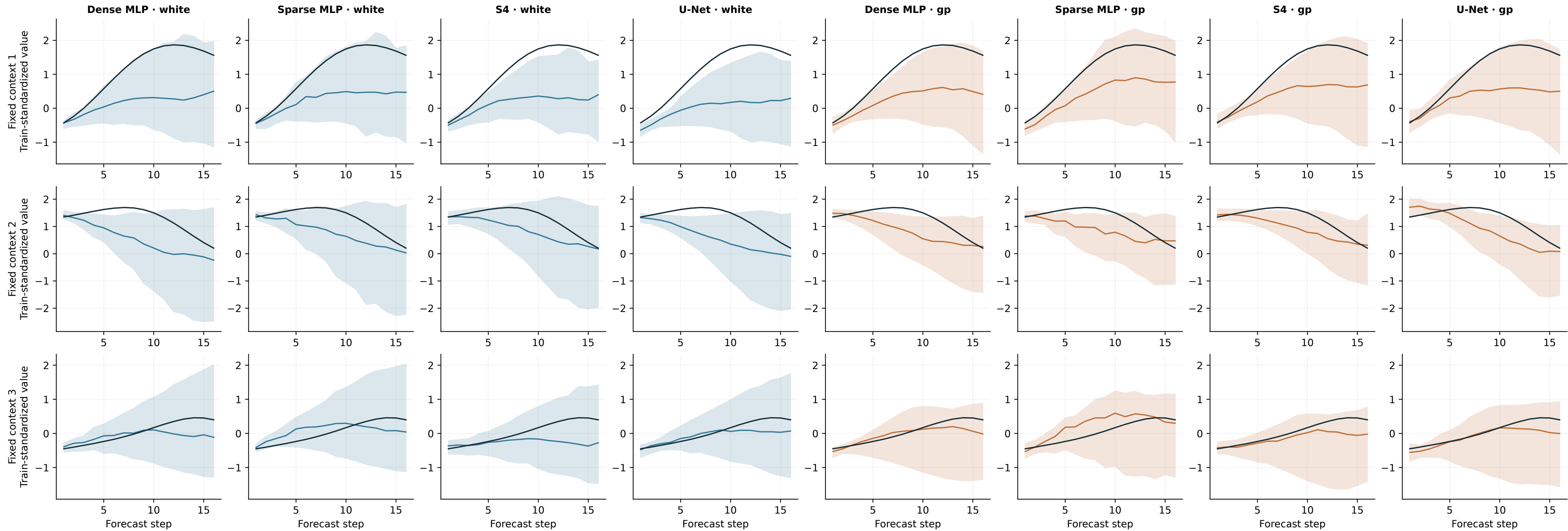
Synthetic GP · 3 channels · channel_2 · first three selected contexts, seed 31 Black: observed future; color: median and marginal 90% band; shared row axes
