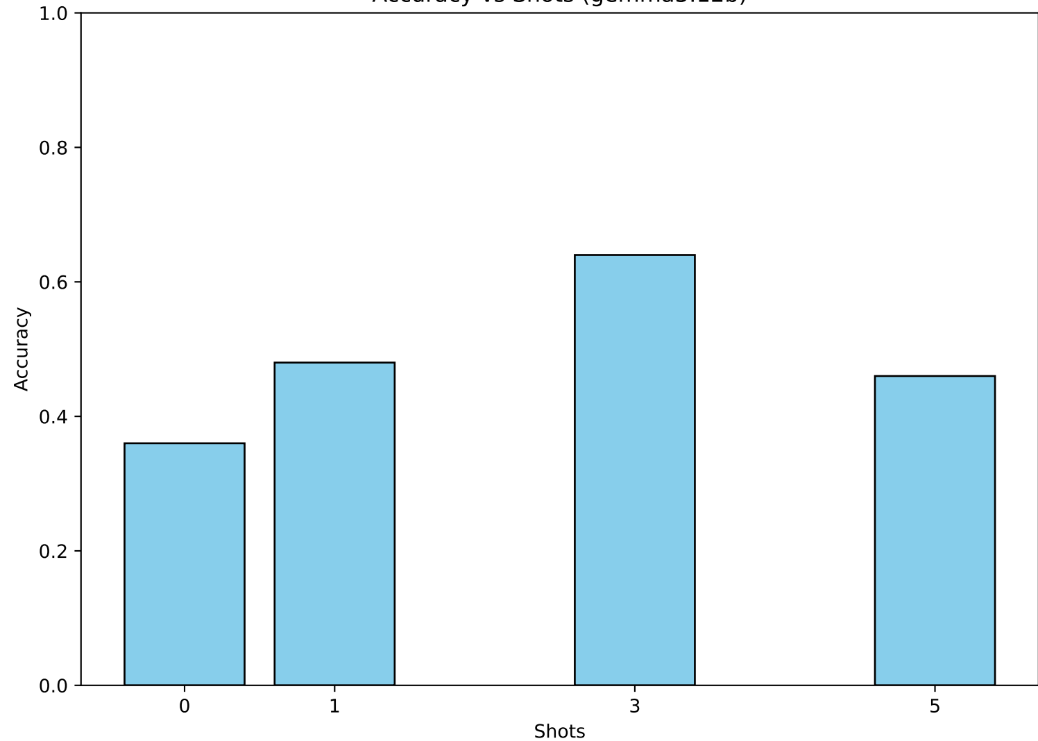
Accuracy vs Shots (gemma3:12b)
