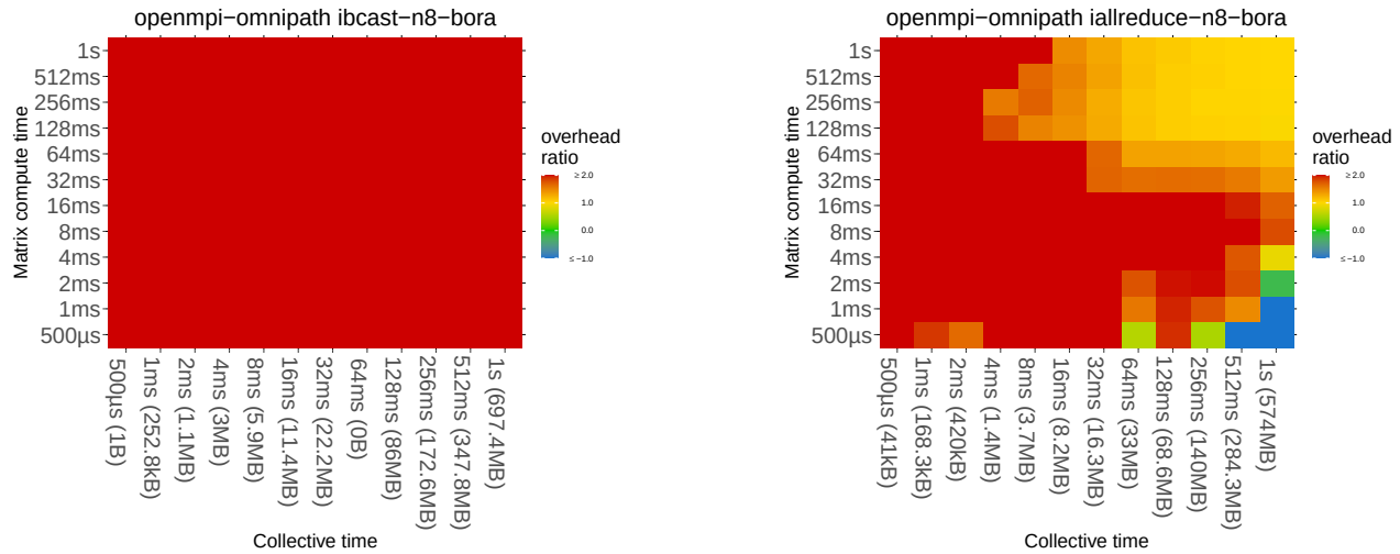
FIGURE 19 OpenMPI 4.0.2 overlap results on Omni-Path for MPI_Ibcast and MPI_Iallreduce on 8 nodes
