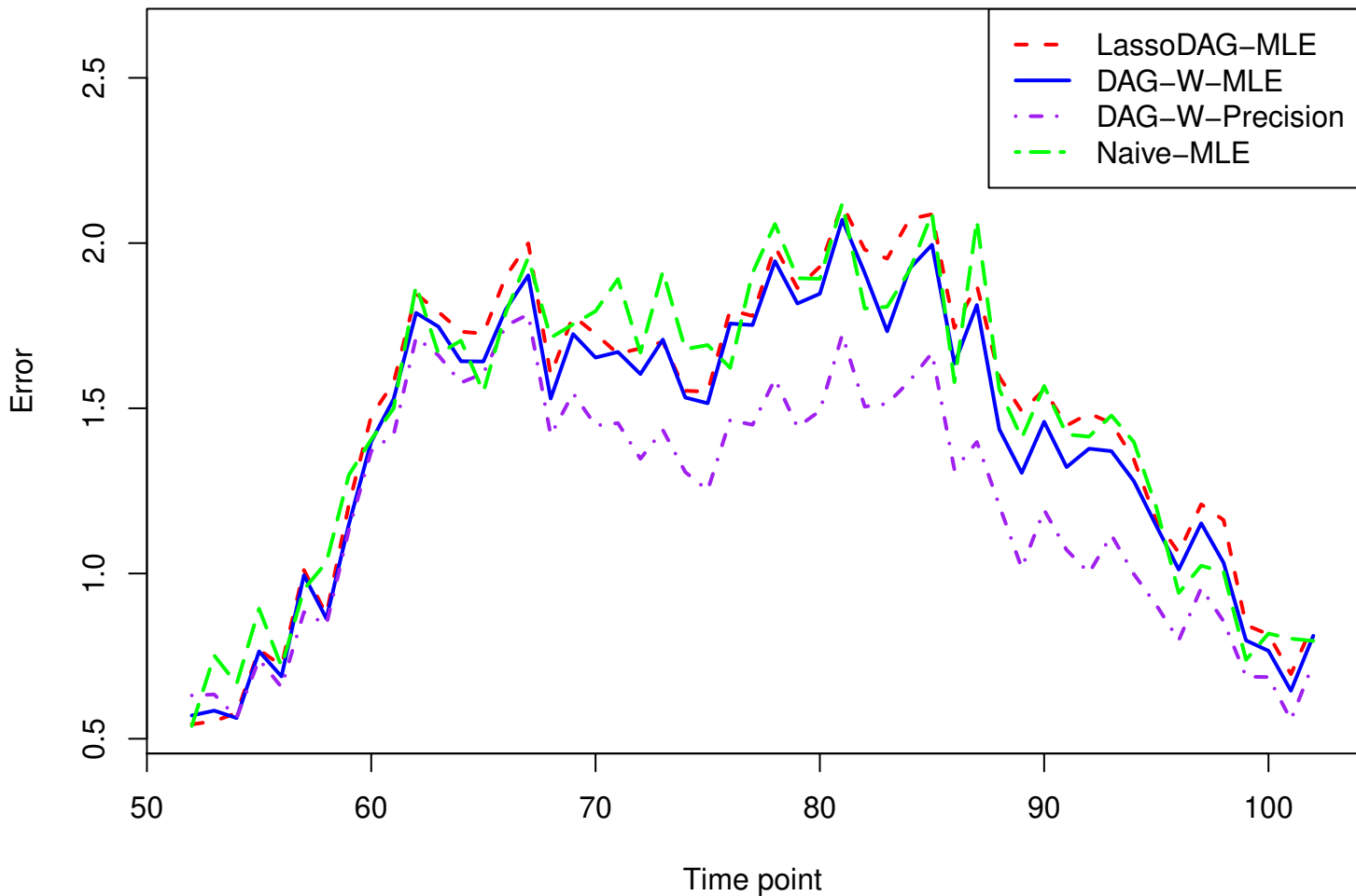
Average Absolute Estimation Error
