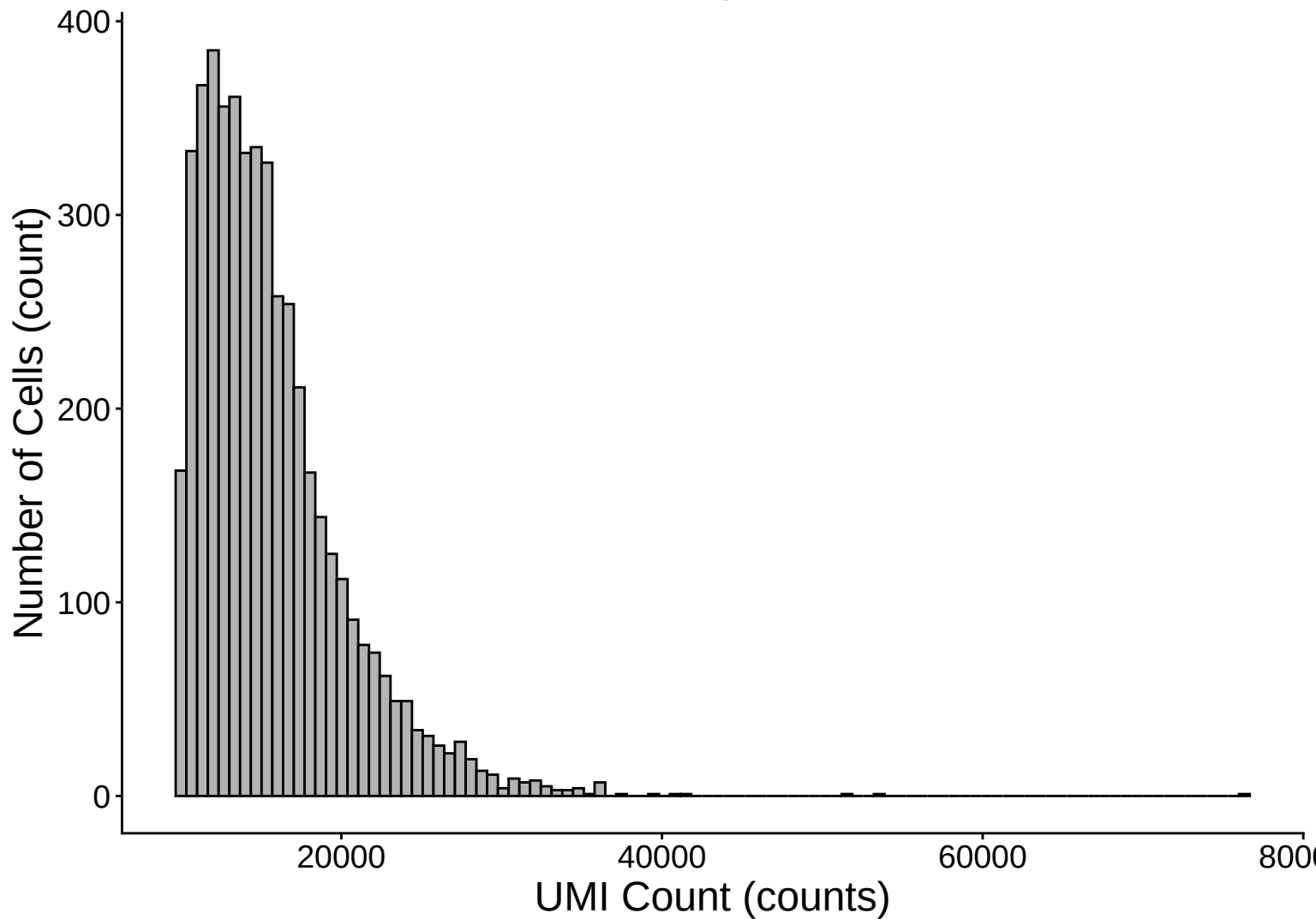
UMI Count Distribution – High Counts (>10,000) – 7dpa
