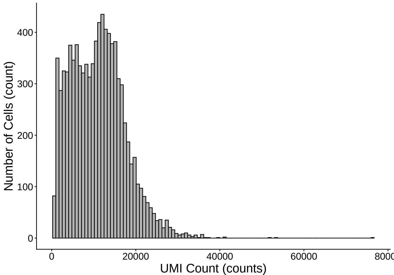
UMI Count per Cell Distribution Histogram – 7dpa
