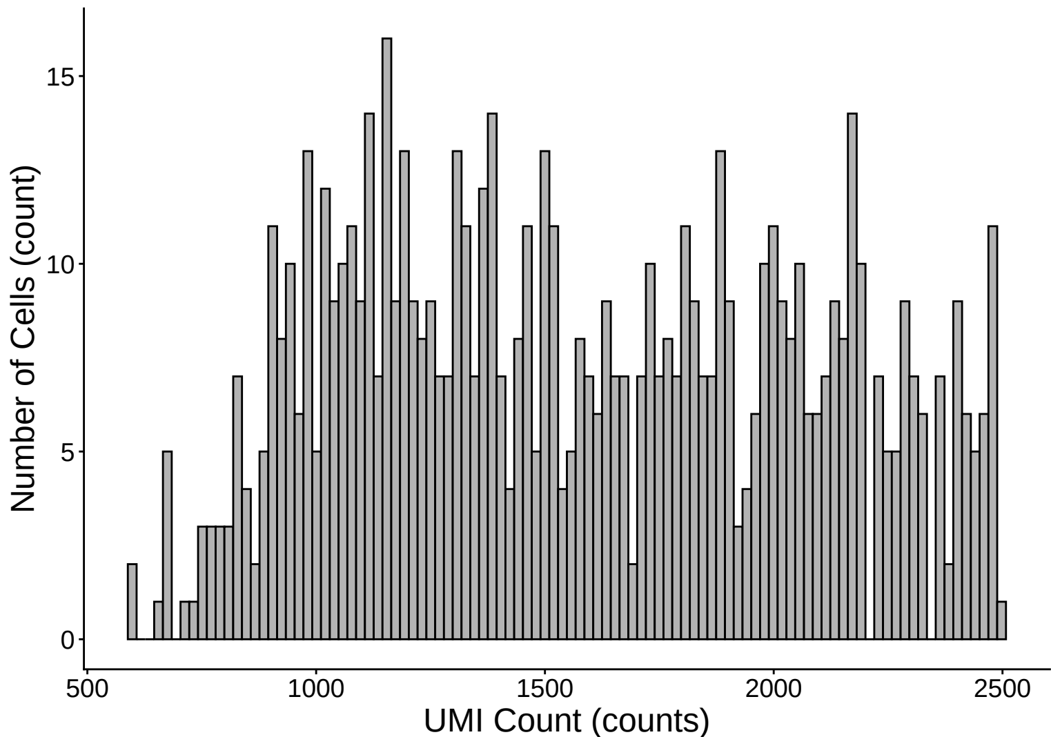
UMI Count Distribution – Low Counts (<2,500) – 7dpa
