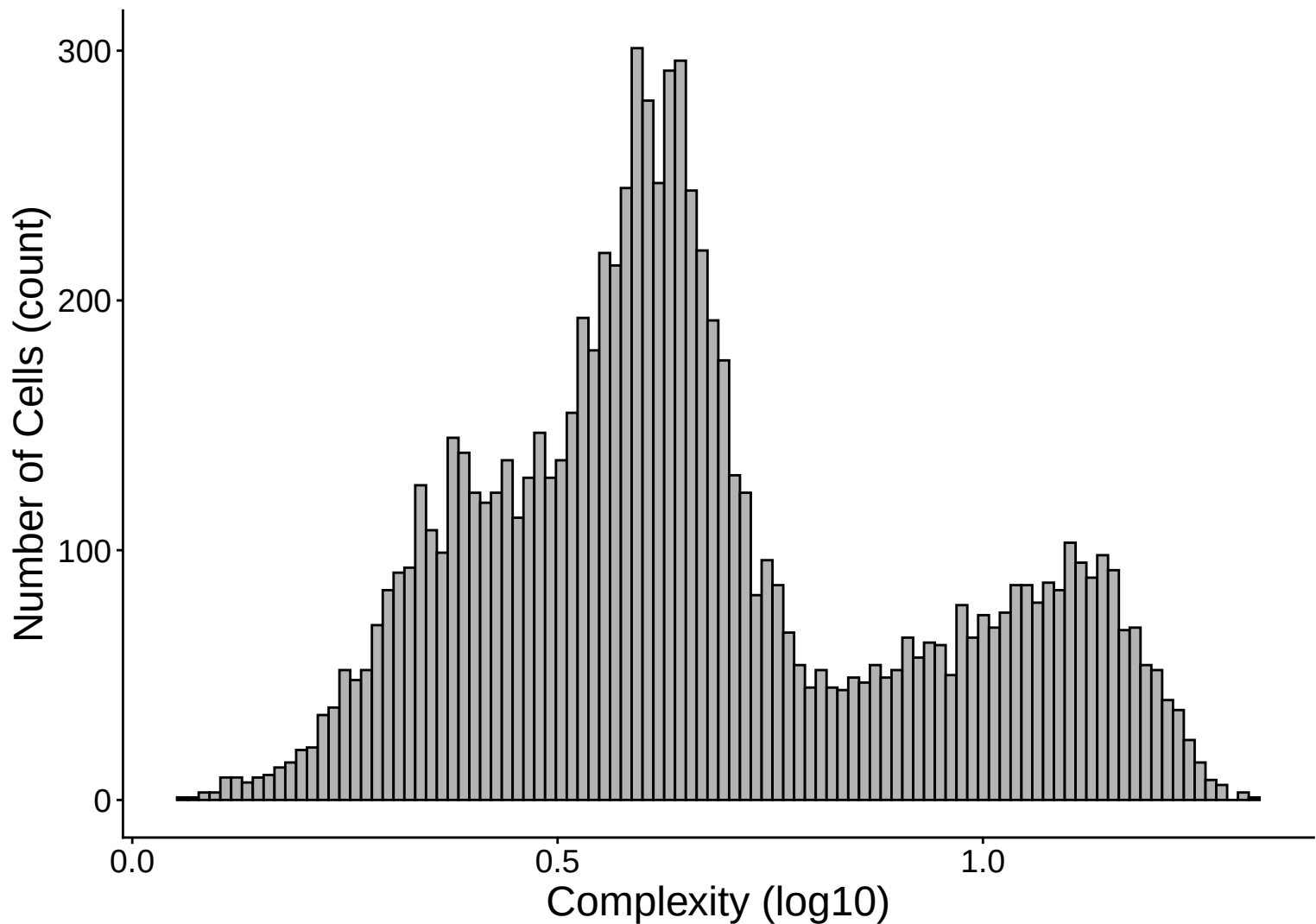
Library Complexity Distribution Histogram – 7dpa
