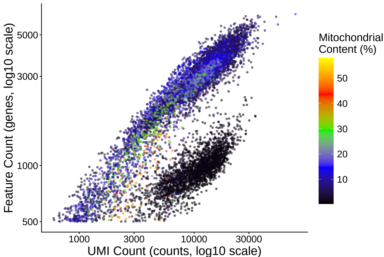
Feature vs UMI Count colored by Mitochondrial Content r = 0.689 - 7\text{dpa}
