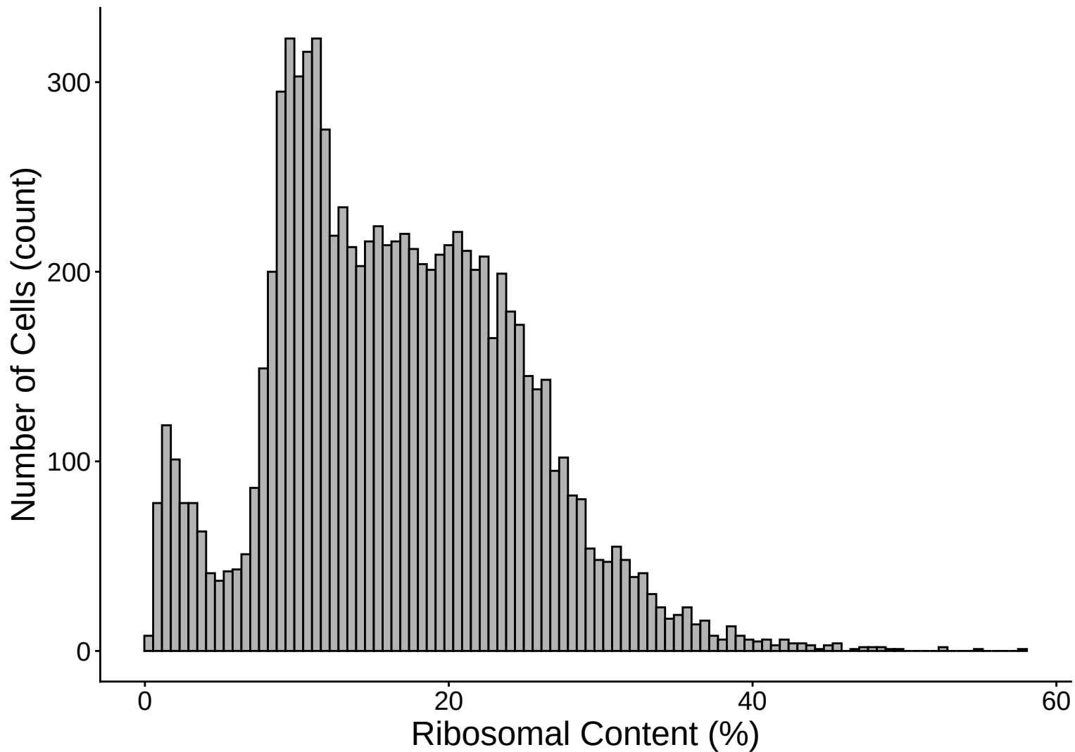
Ribosomal Percentage Distribution Histogram – 7dpa
