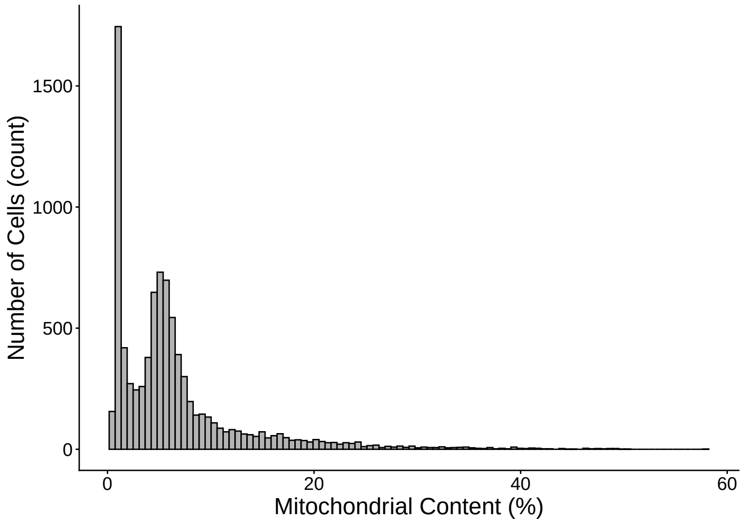
Mitochondrial Percentage Distribution Histogram – 7dpa
