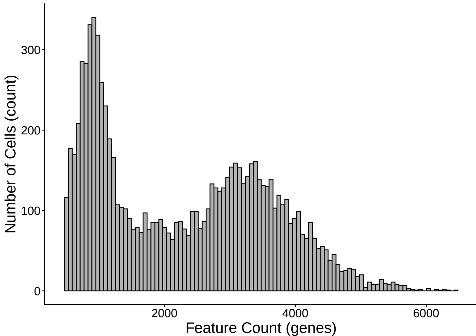
Feature Count per Cell Distribution Histogram – 7dpa
