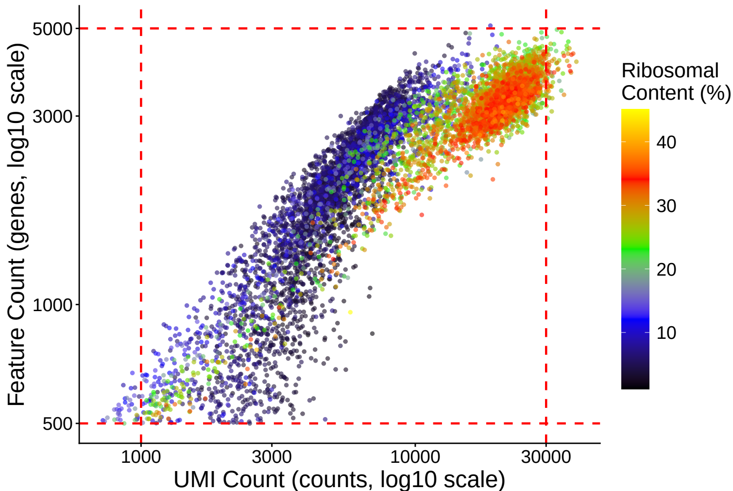
Feature vs UMI Count colored by Ribosomal Content r = 0.844 - 22\text{dpa}
