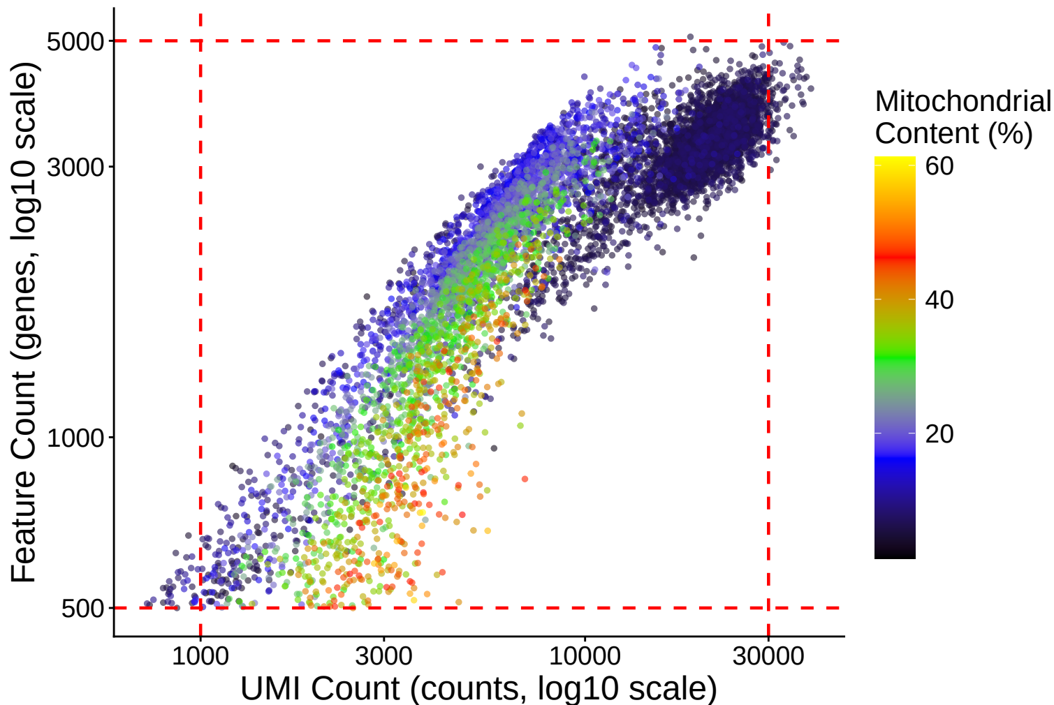
Feature vs UMI Count colored by Mitochondrial Content r = 0.844 - 22\text{dpa}
