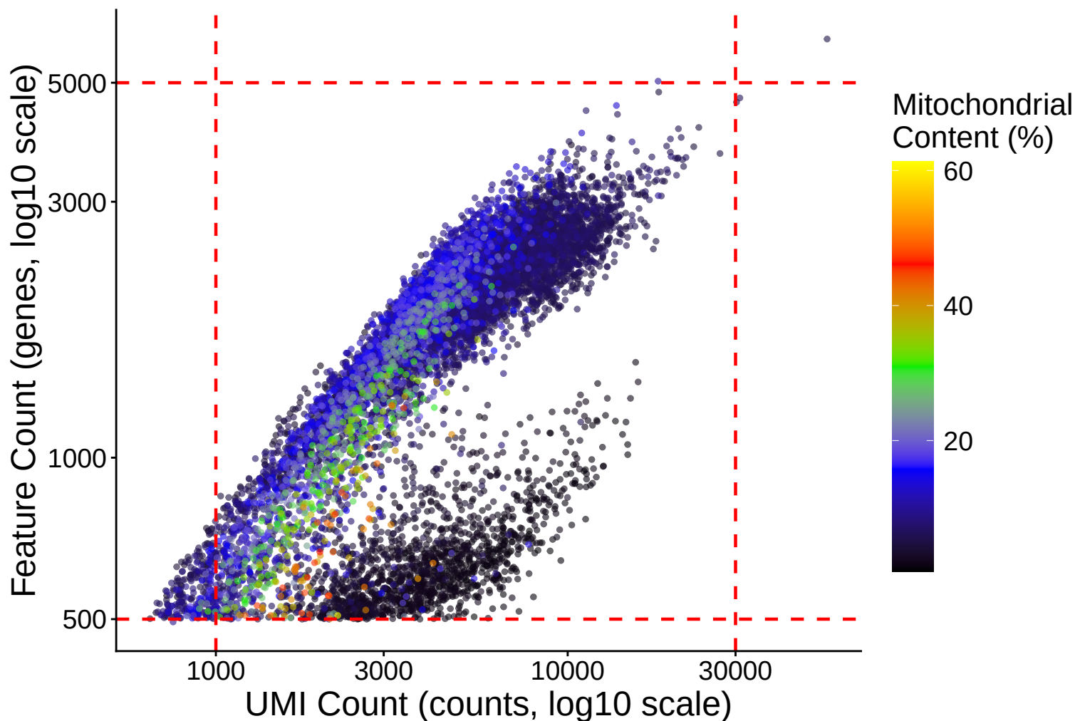
Feature vs UMI Count colored by Mitochondrial Content r = 0.733 - 72h
