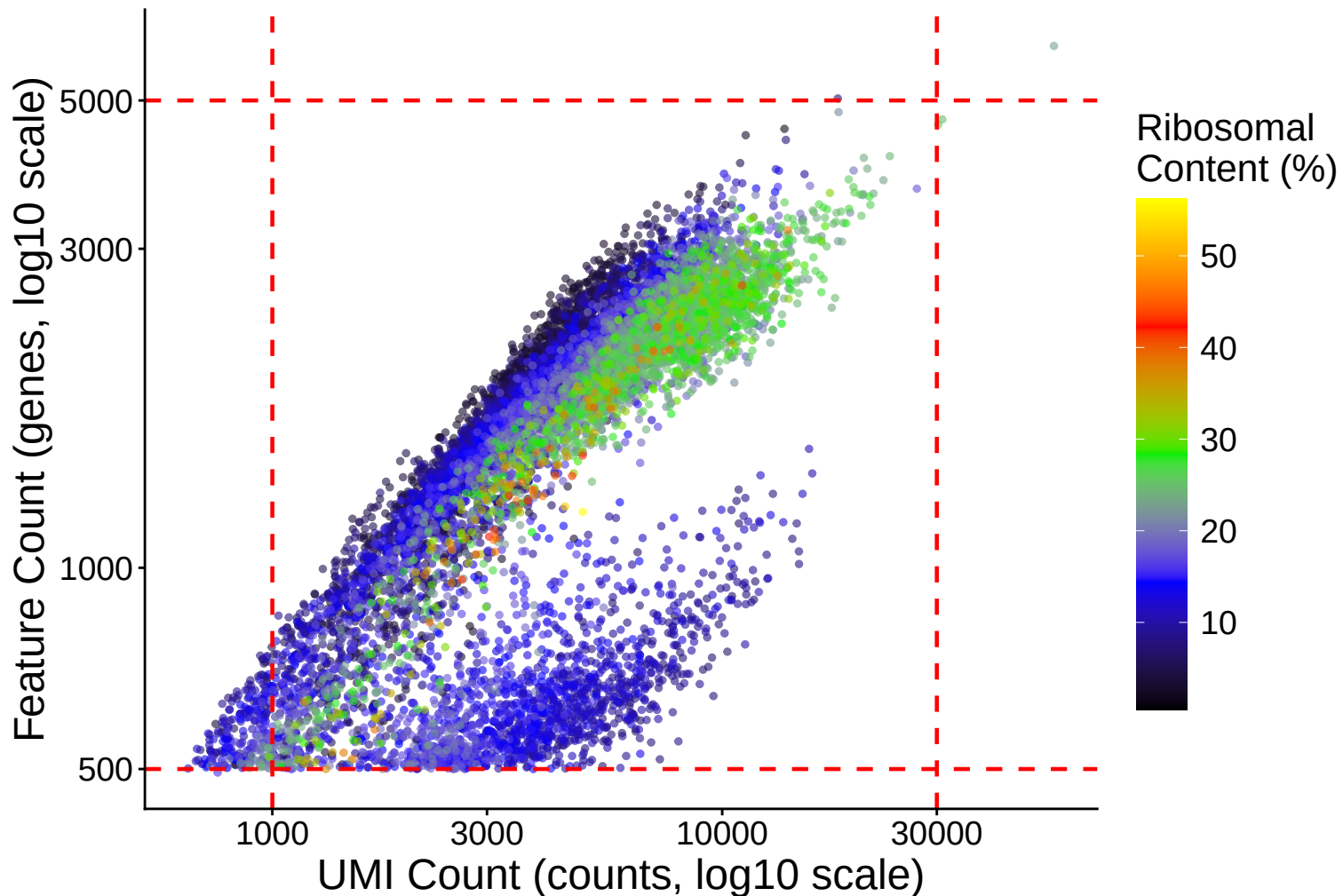
Feature vs UMI Count colored by Ribosomal Content r = 0.733 - 72h
