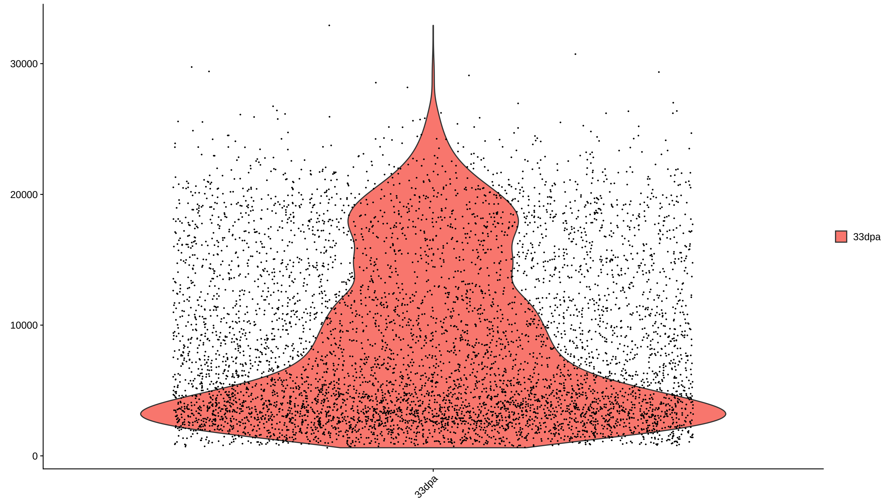
nCount_RNA
