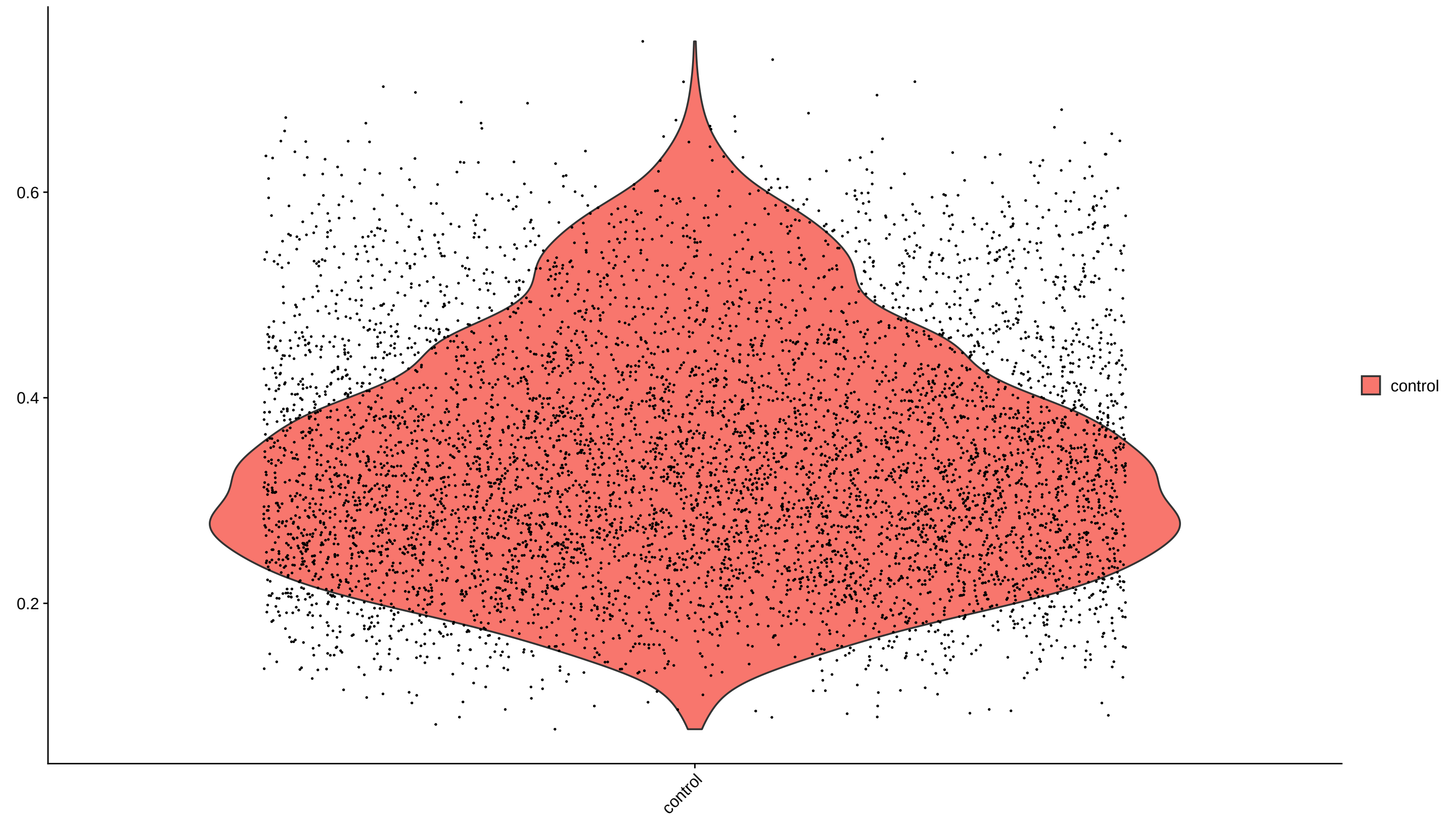
log10UMIsPerGene
