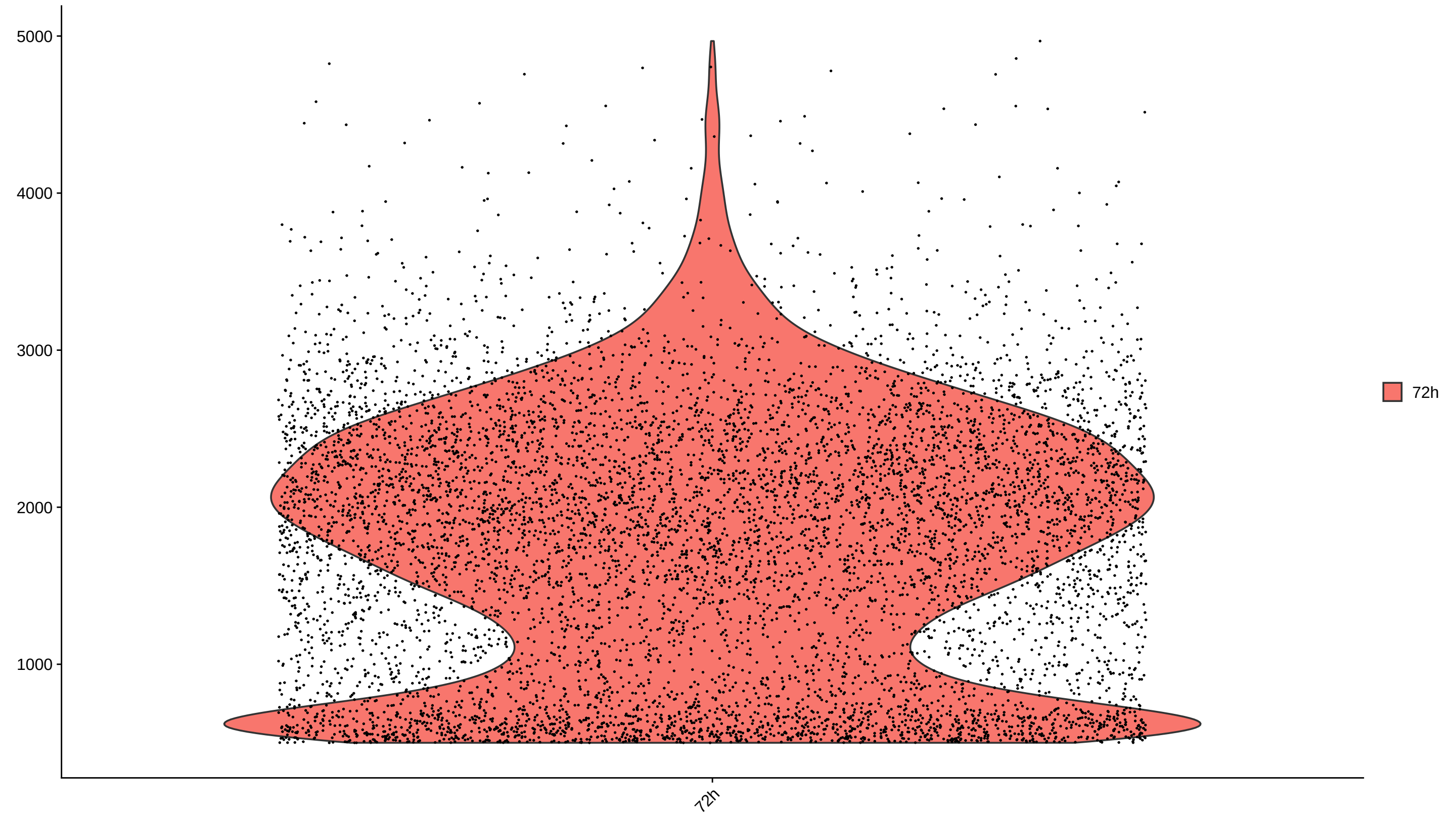
nFeature_RNA
