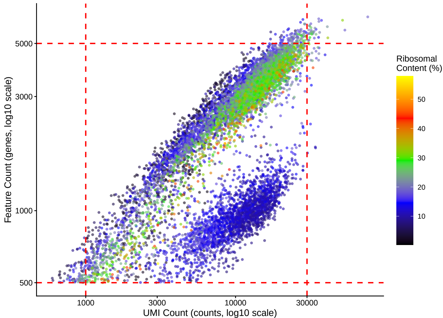
Feature vs UMI Count colored by Ribosomal Content – r = 0.689 – 7dpa
