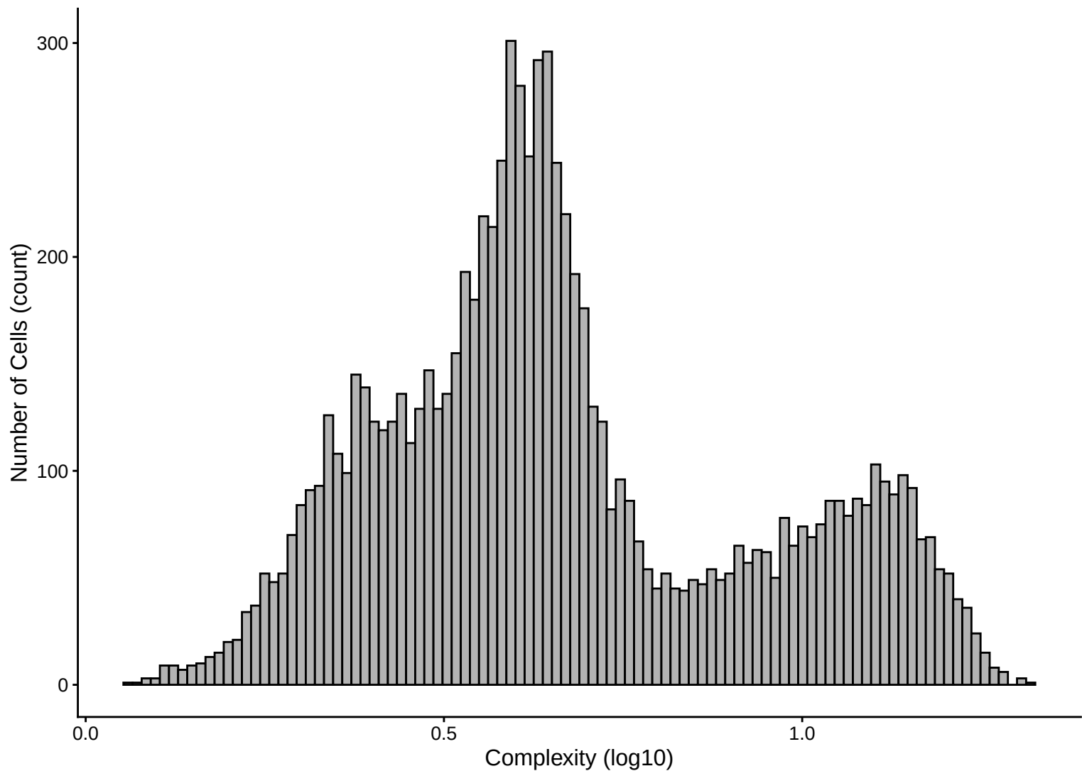
Library Complexity Distribution – Histogram – 7dpa
