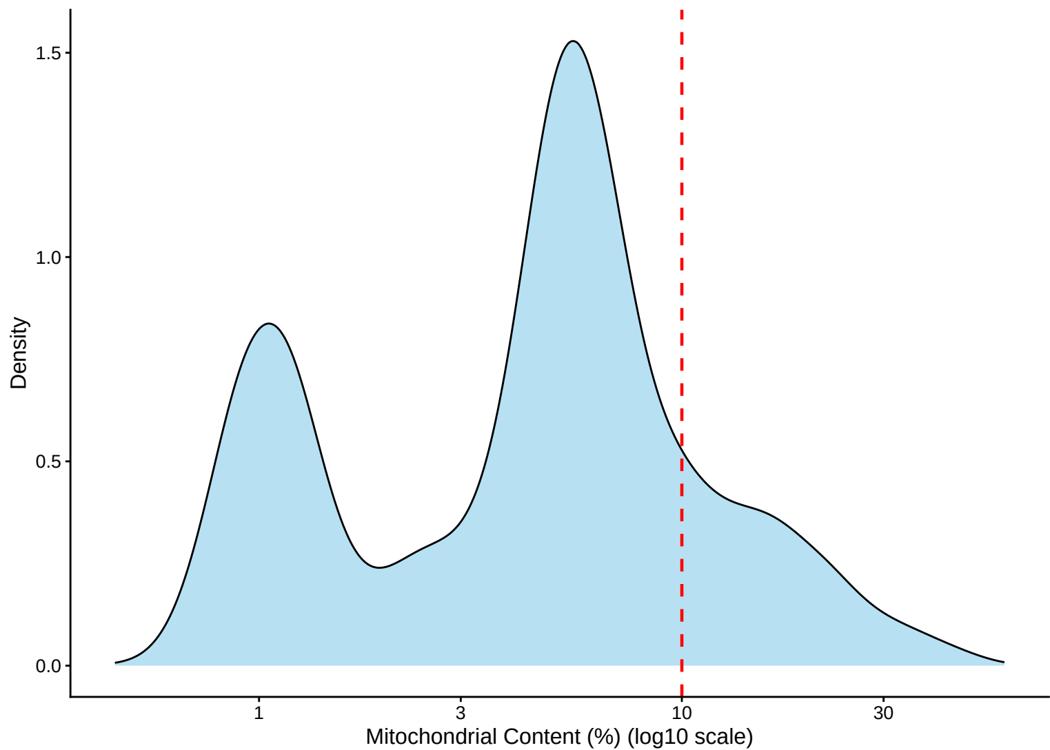
Mitochondrial Percentage Distribution – Kernel Density Estimate – 7dpa
