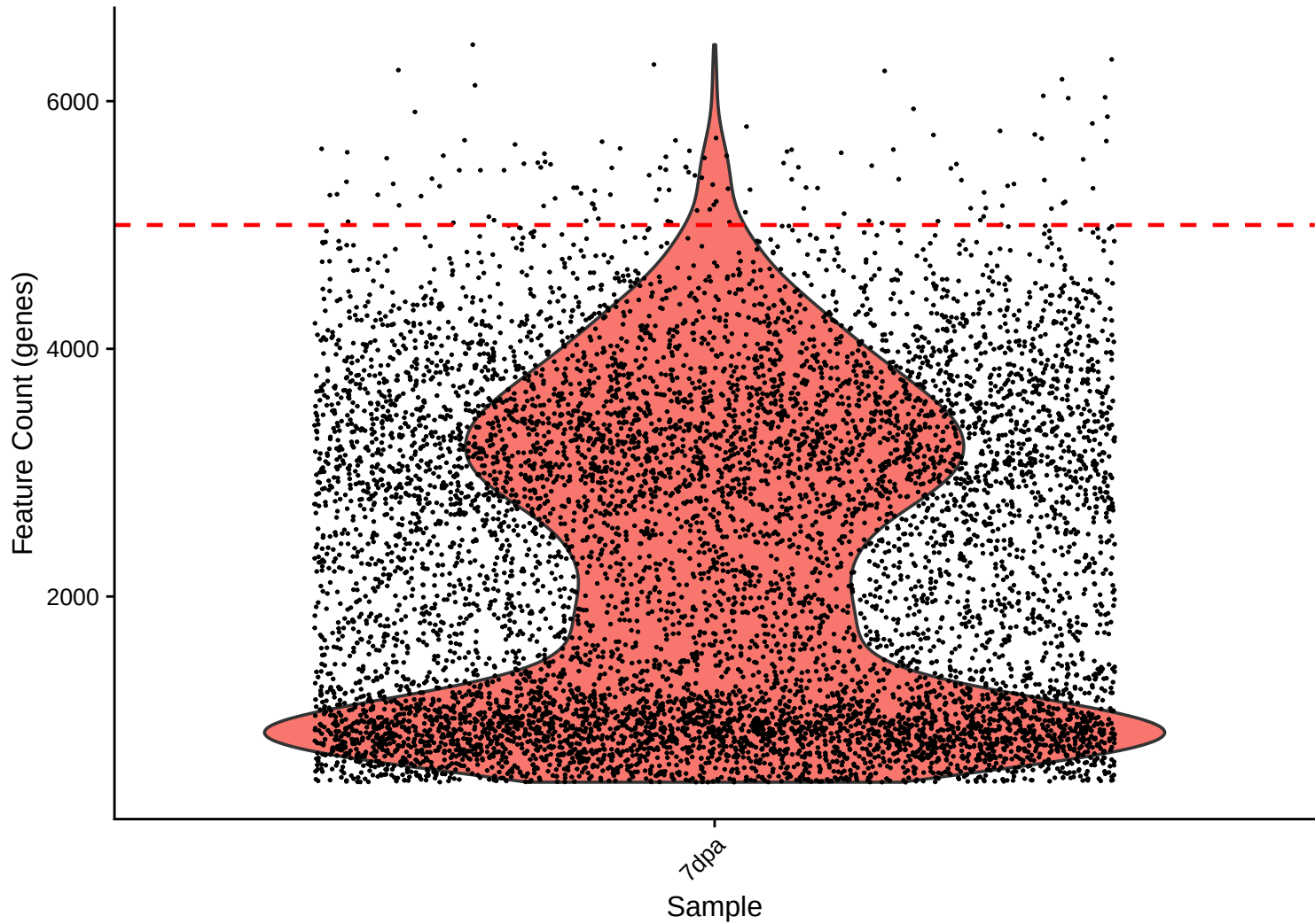
Feature Count per Cell Distribution – 7dpa
