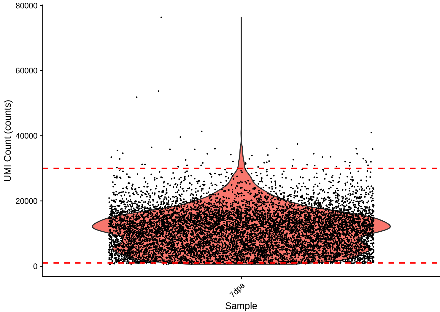
UMI Count per Cell Distribution – 7dpa
