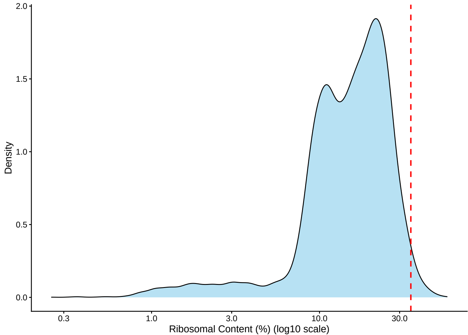
Ribosomal Percentage Distribution – Kernel Density Estimate – 7dpa
