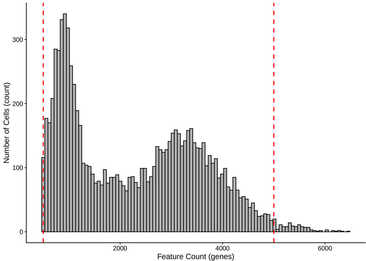
Feature Count per Cell Distribution – Histogram – 7dpa
