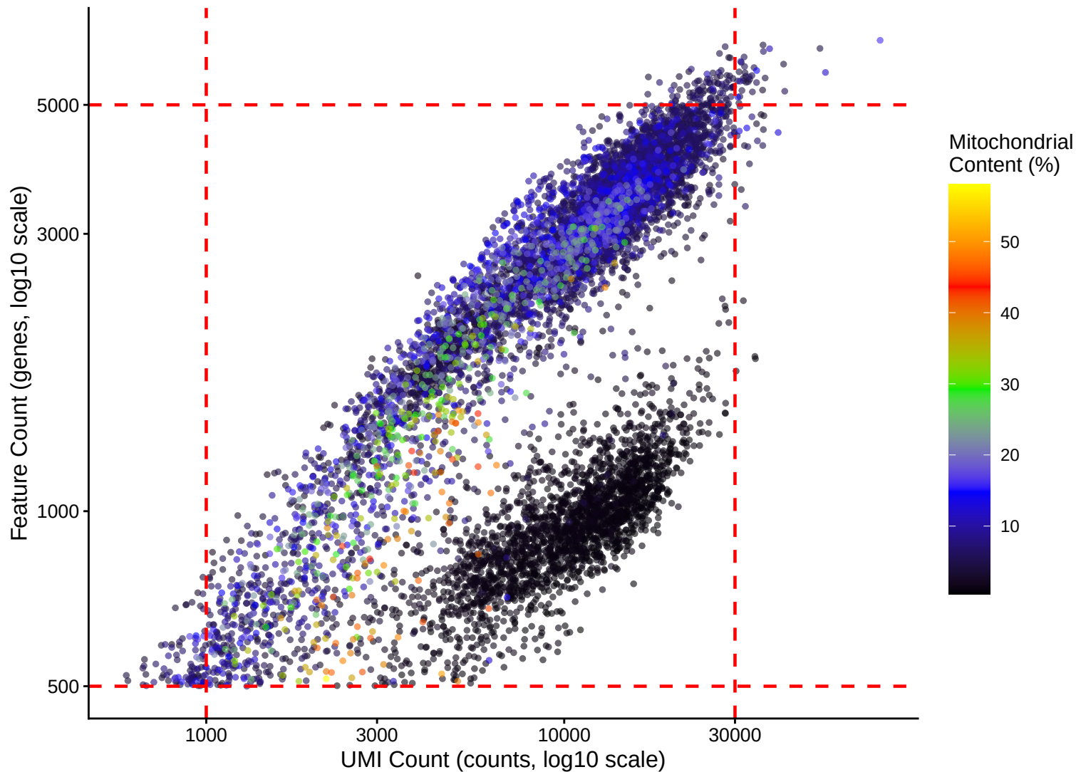
Feature vs UMI Count colored by Mitochondrial Content – r = 0.689 – 7dpa
