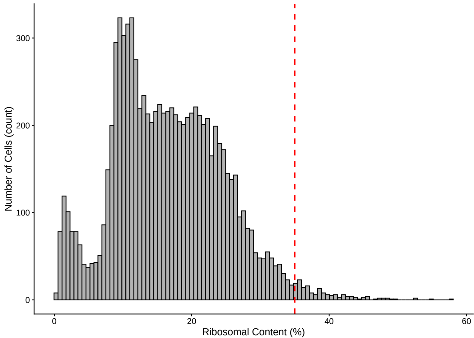
Ribosomal Percentage Distribution – Histogram – 7dpa
