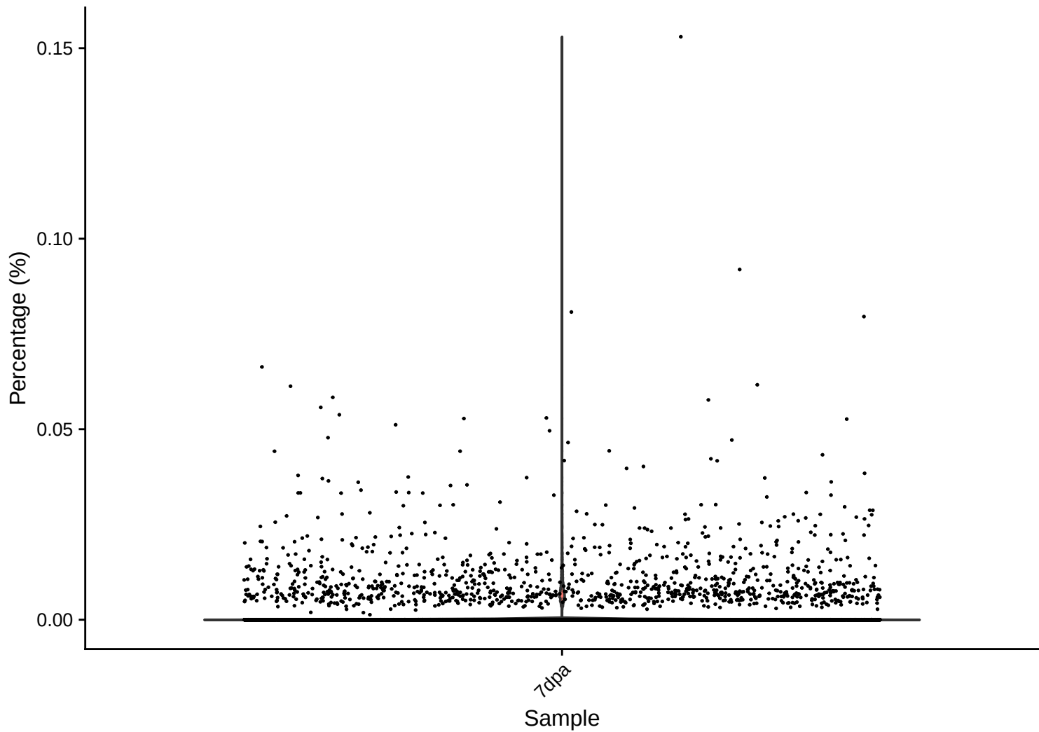
rrna Distribution – 7dpa
