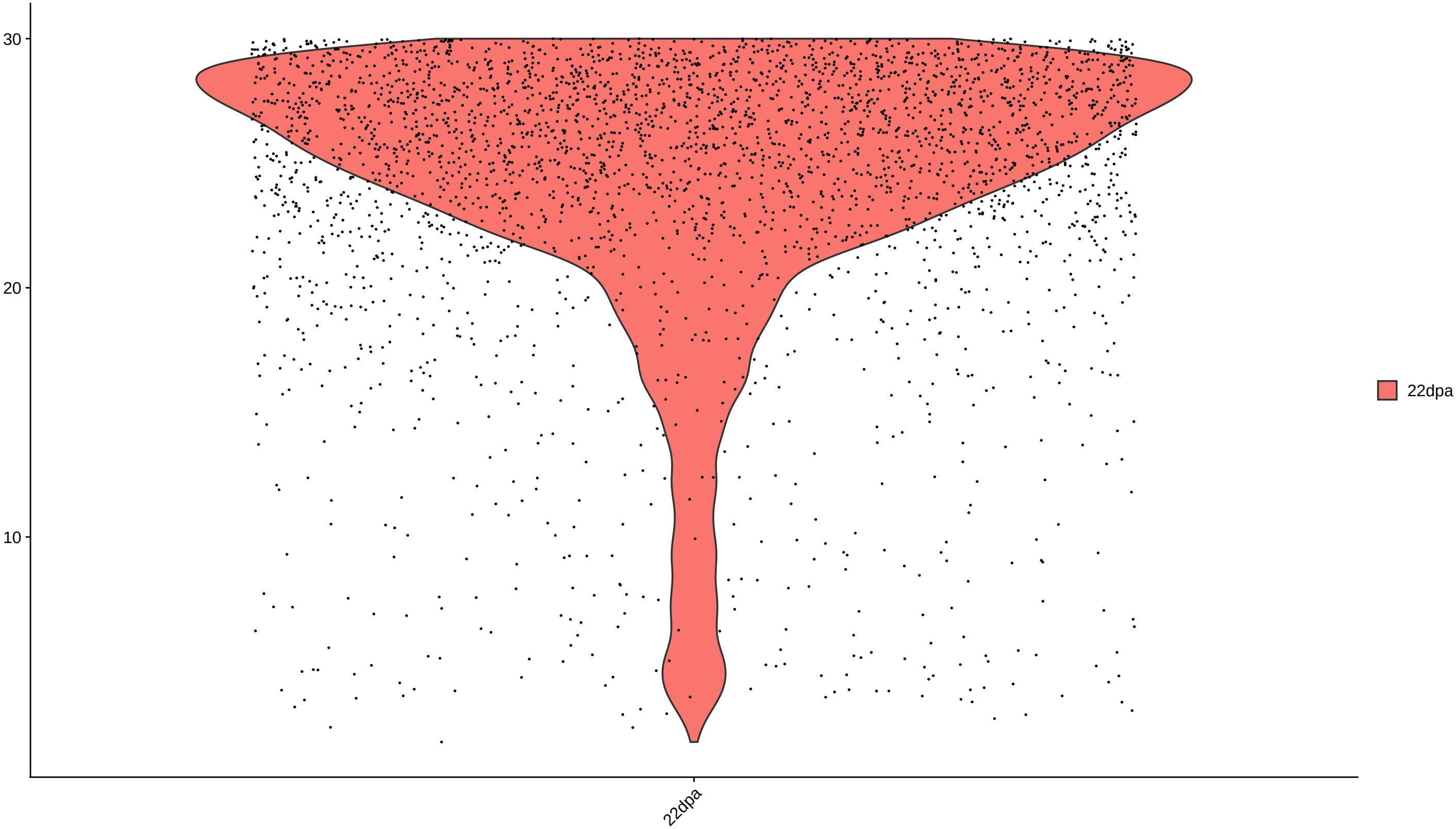
percent.ribo
