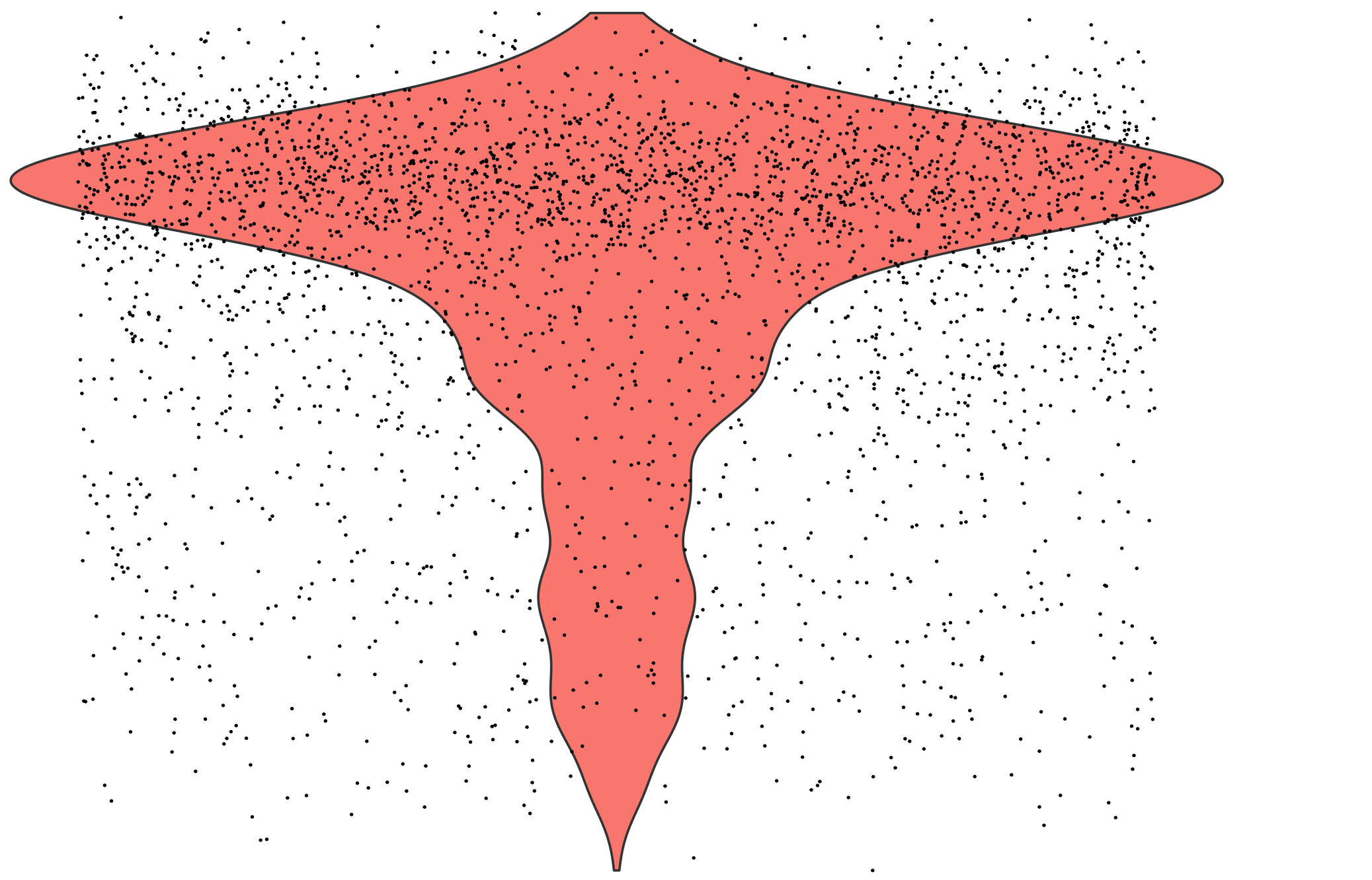
log10UMIsPerGene
