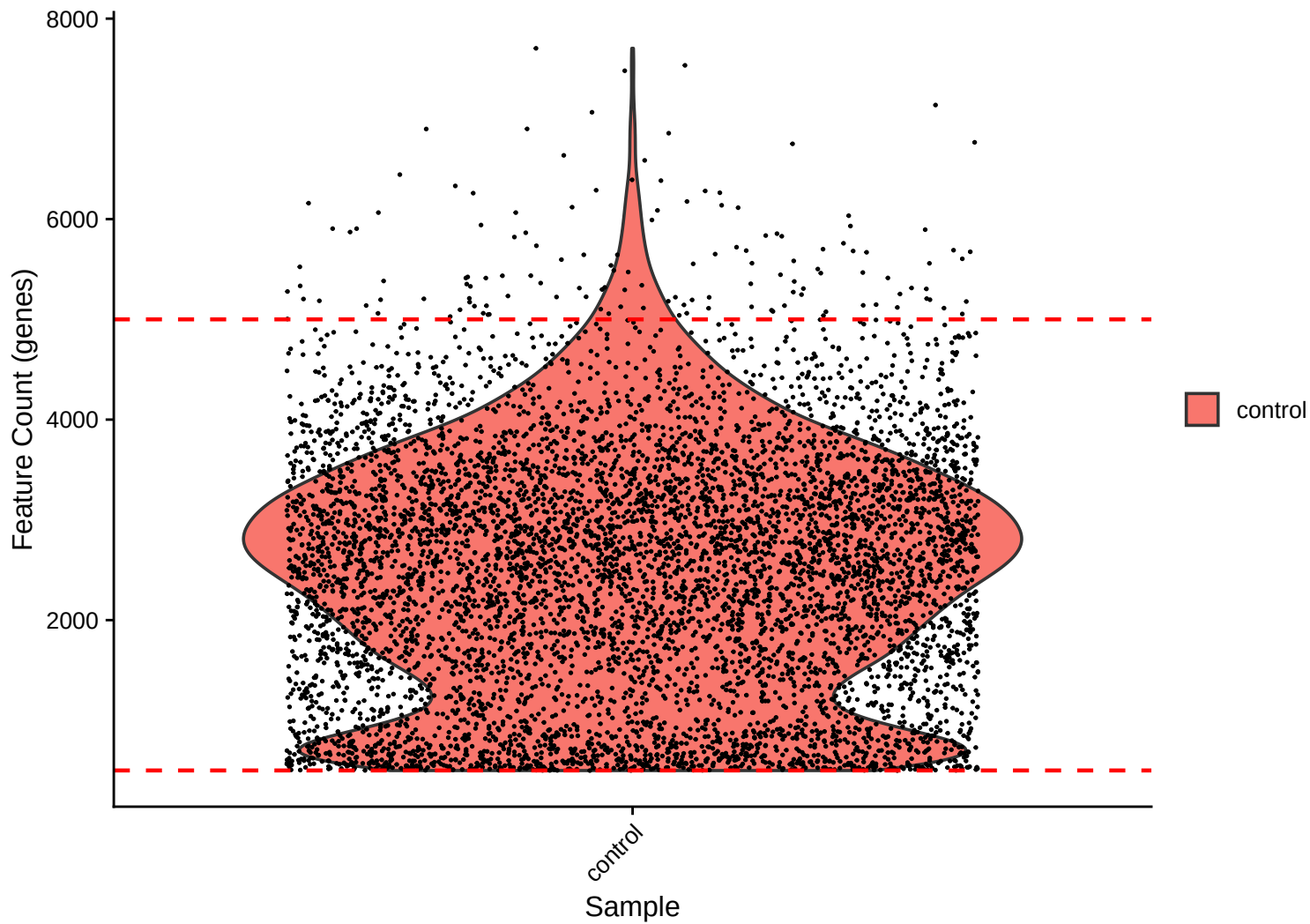
Feature Count per Cell Distribution
