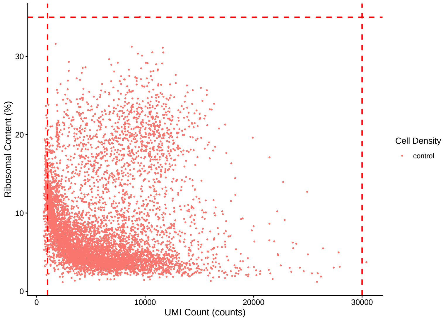
Ribosomal Content (%) vs UMI Count
