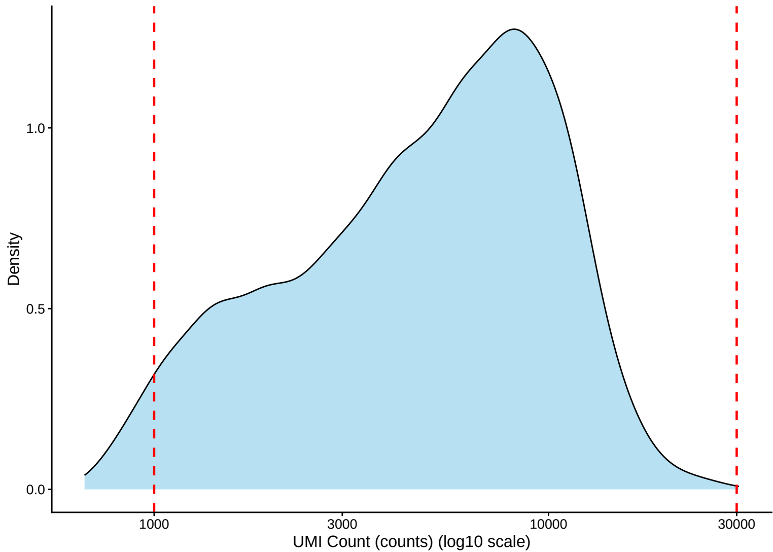
UMI Count per Cell Distribution – Kernel Density Estimate
