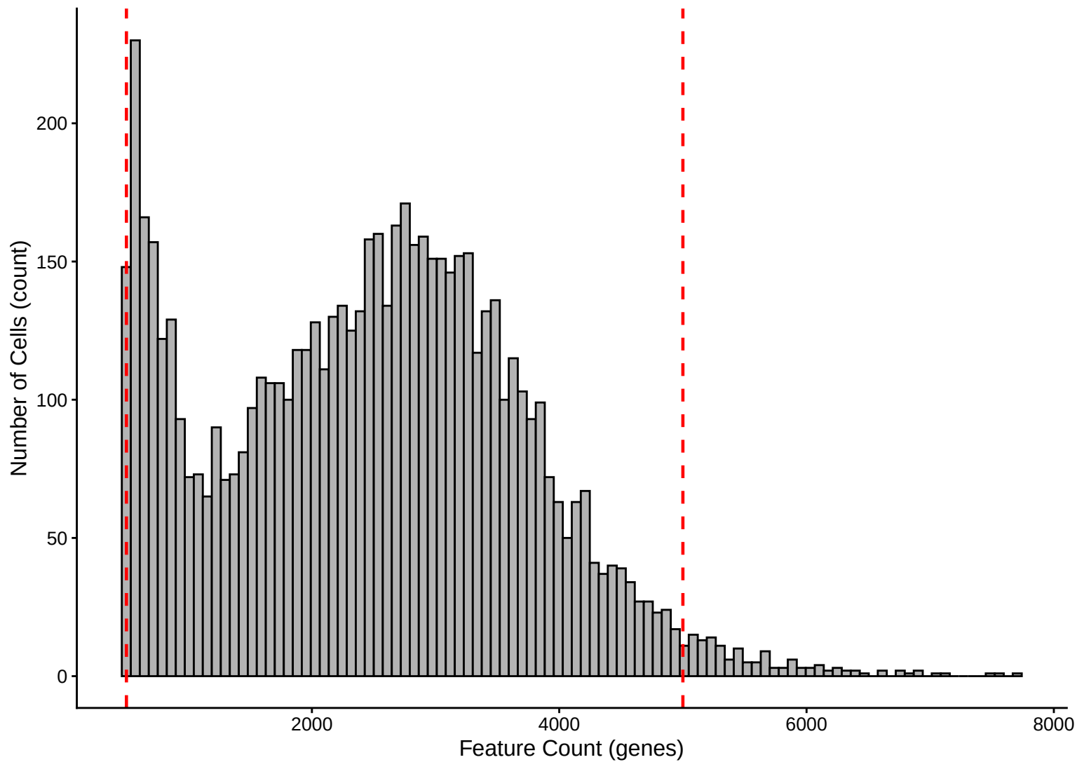
Feature Count per Cell Distribution – Histogram
