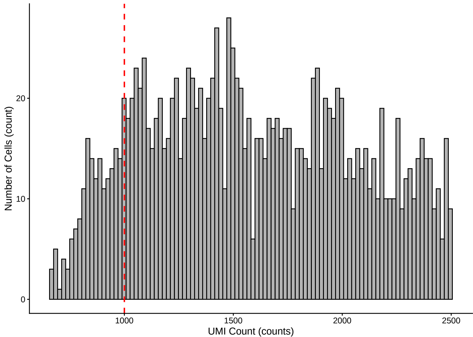
UMI Count Distribution – Low Counts (<2,500)
