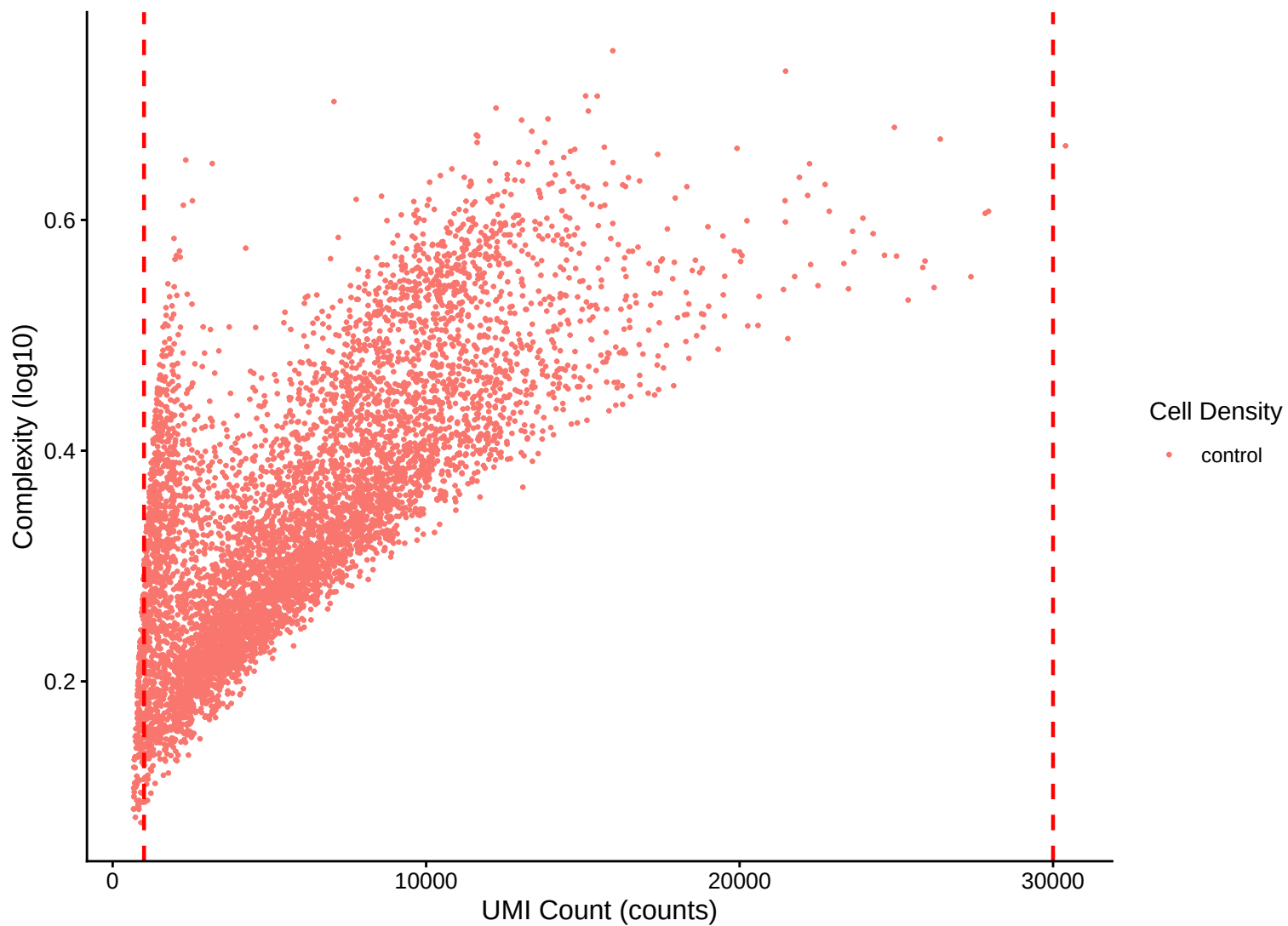
Complexity (log10) vs UMI Count
