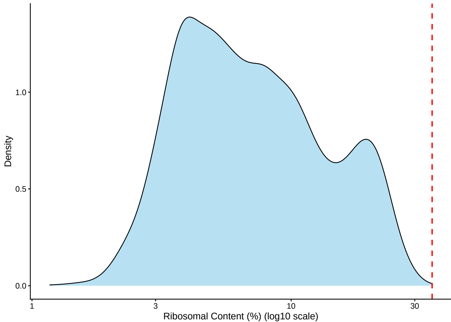
Ribosomal Percentage Distribution – Kernel Density Estimate
