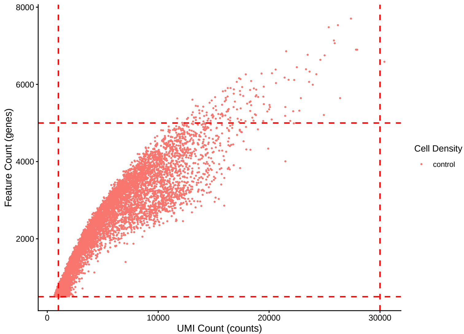
Feature Count (genes) vs UMI Count
