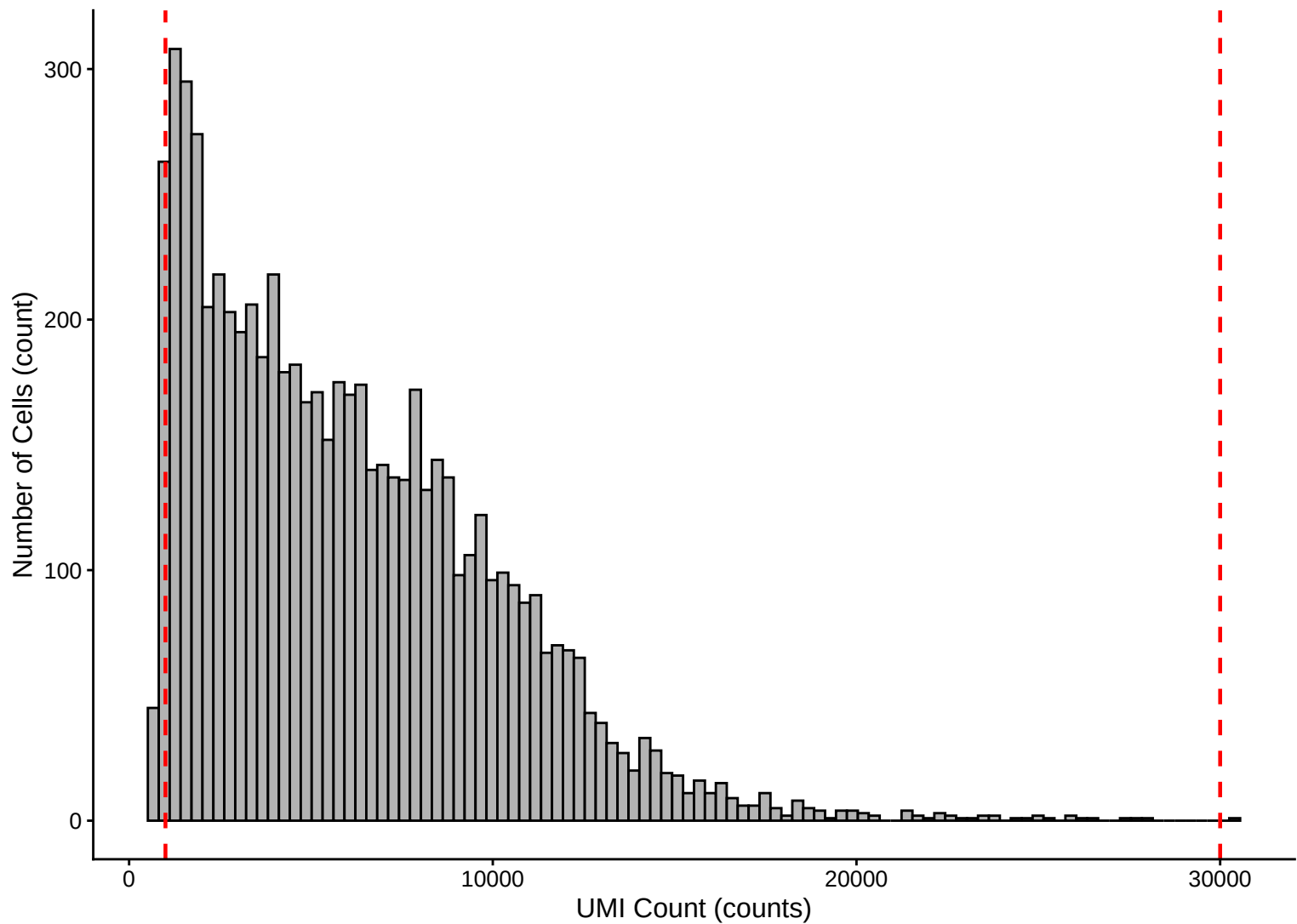
UMI Count per Cell Distribution – Histogram
