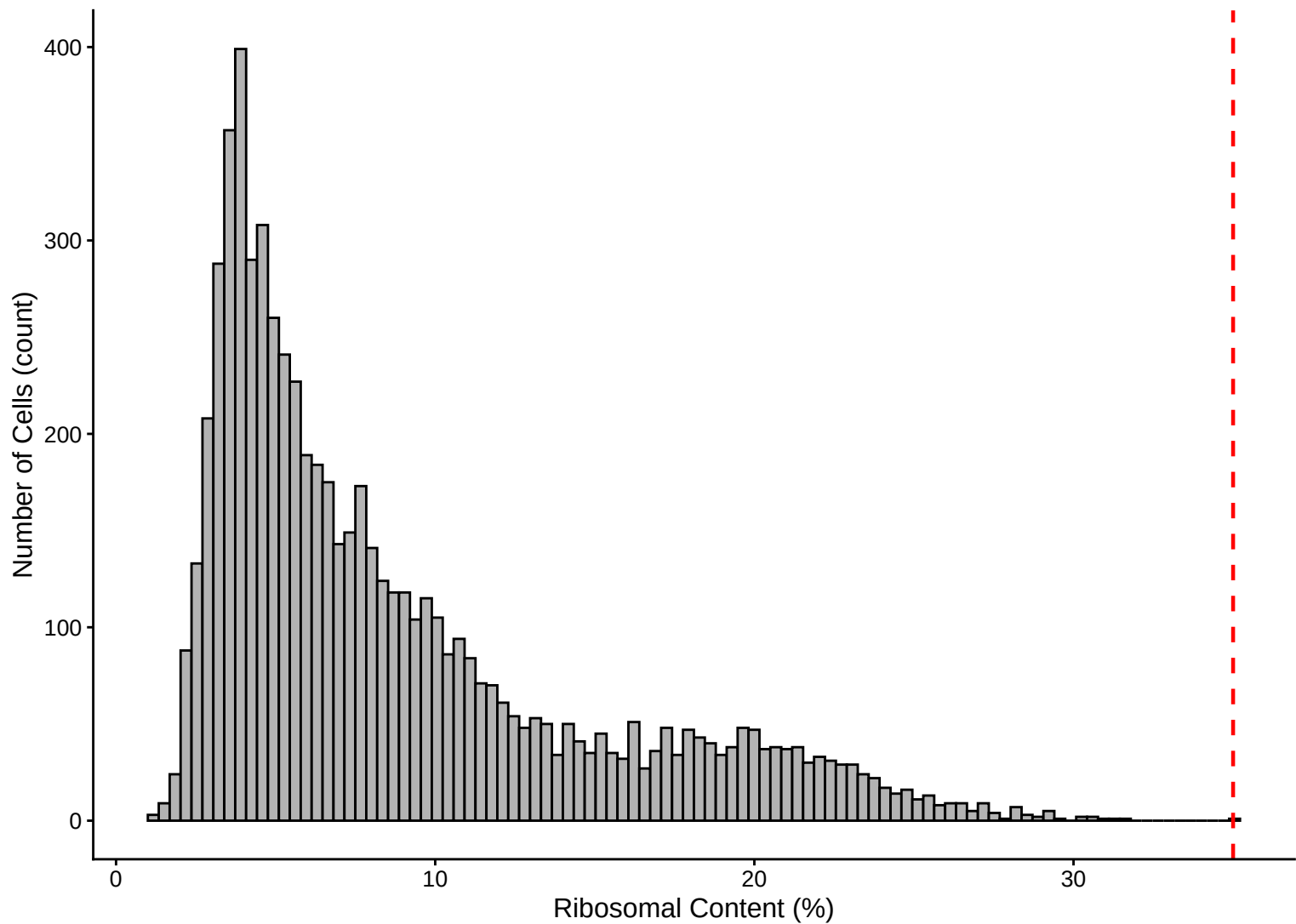
Ribosomal Percentage Distribution – Histogram
