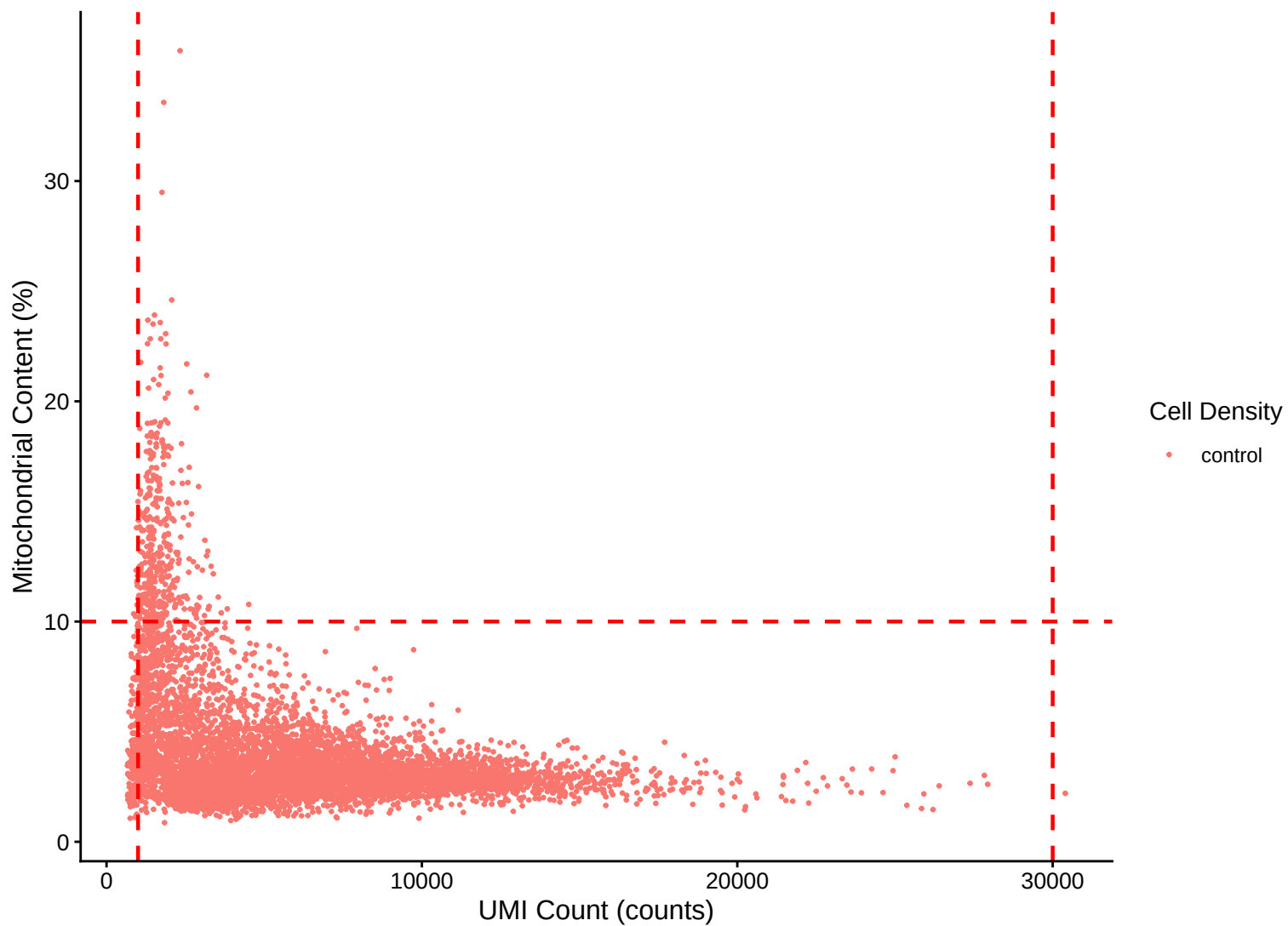
Mitochondrial Content (%) vs UMI Count
