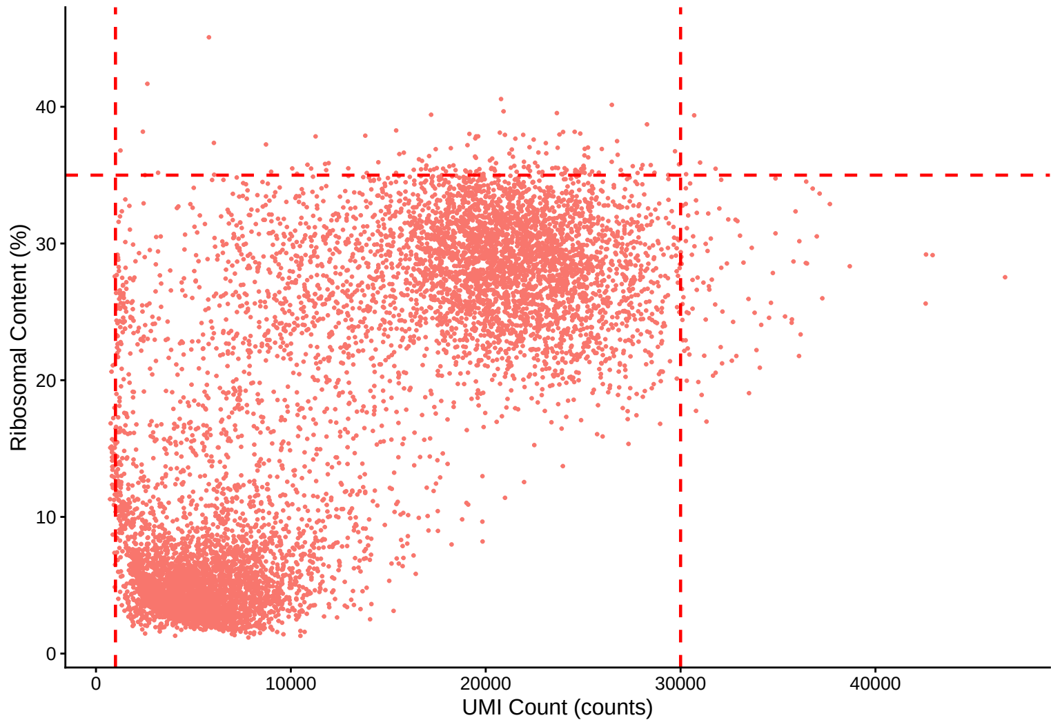
Ribosomal Content (%) vs UMI Count r = 0.778 - 22\text{dpa}
