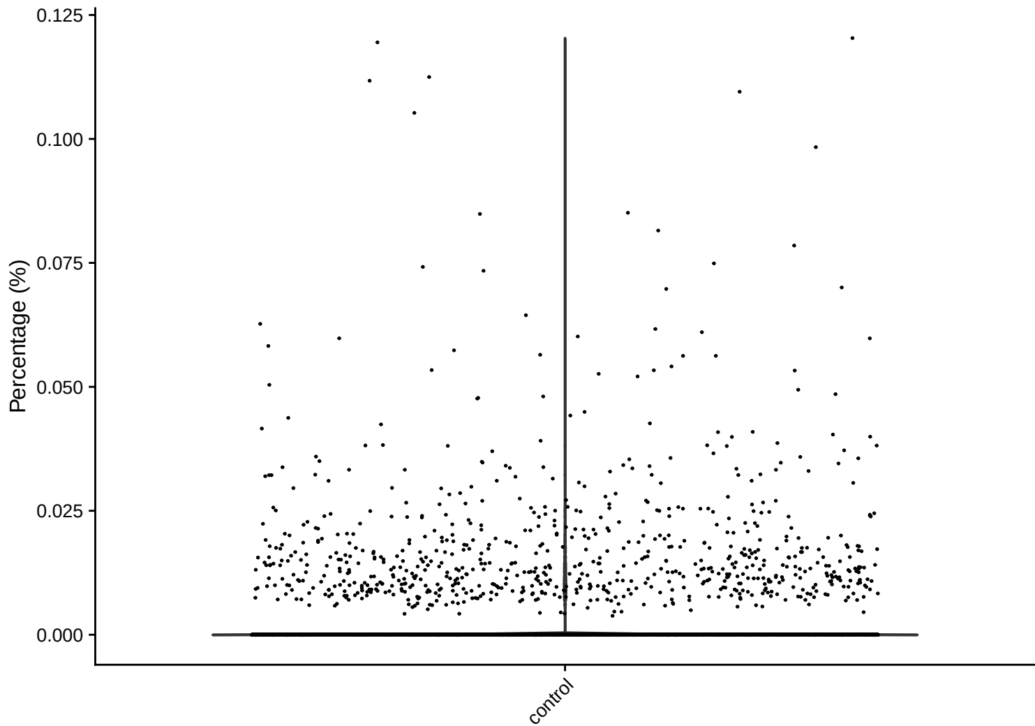
trna Distribution – control
