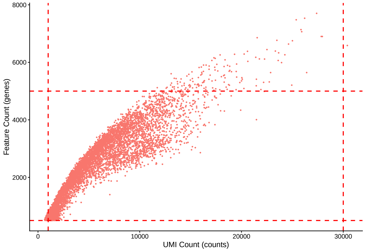
Feature Count (genes) vs UMI Count r = 0.91 – control
