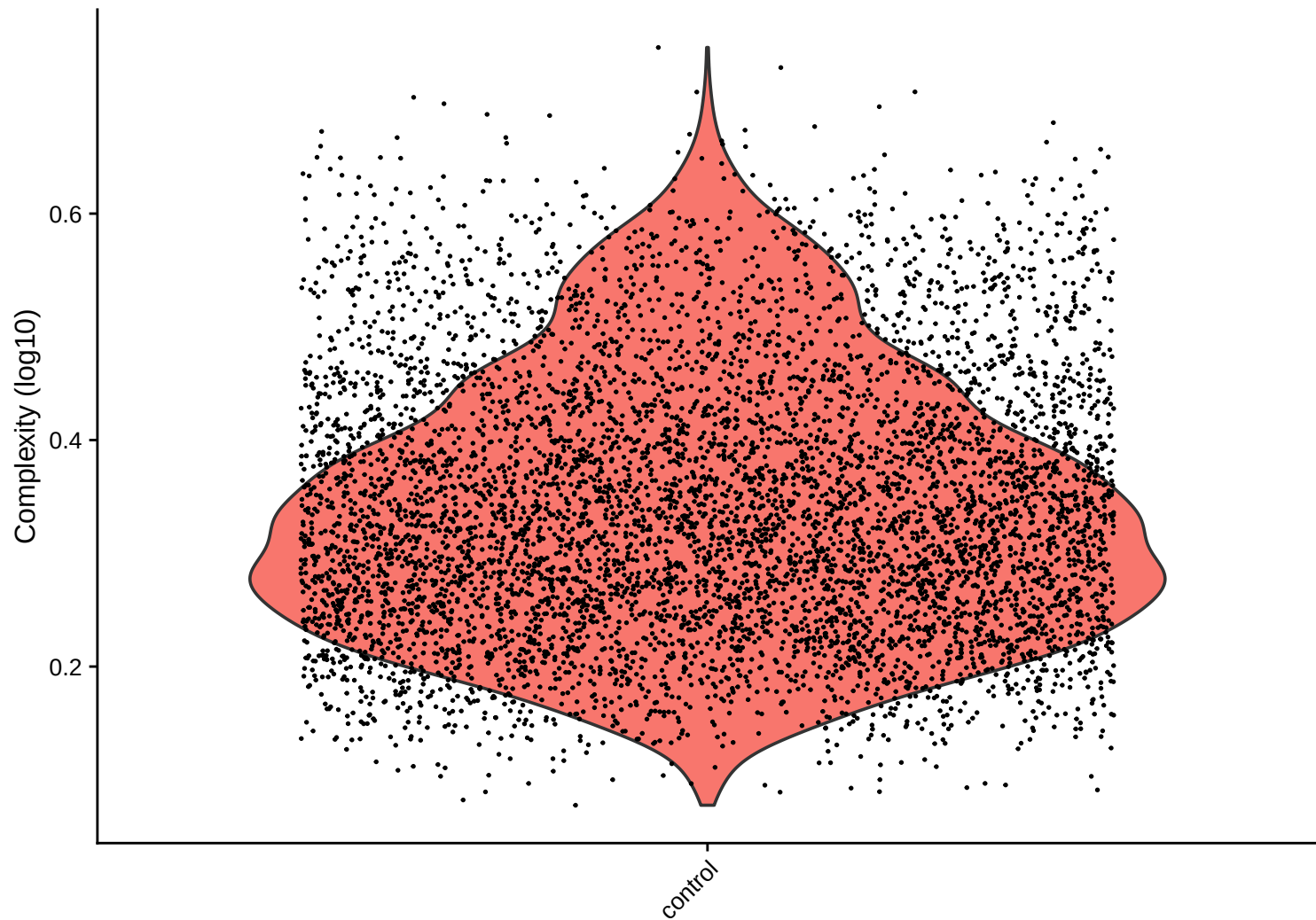
Library Complexity Distribution – control
