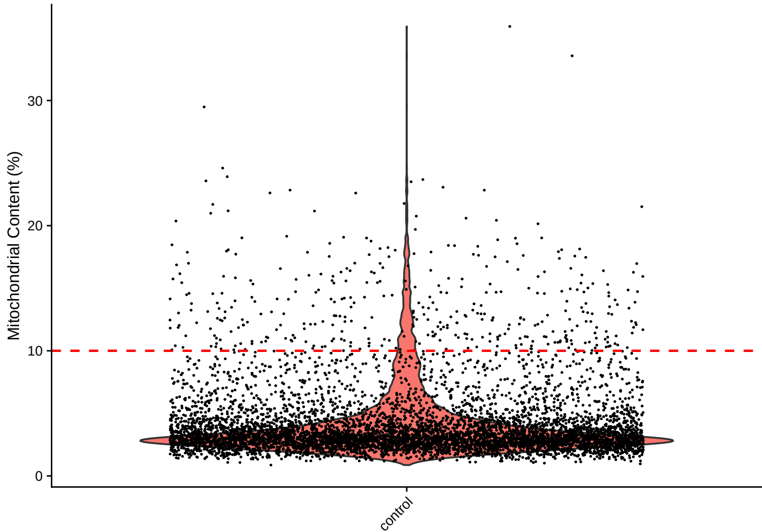
Mitochondrial Percentage Distribution – control
