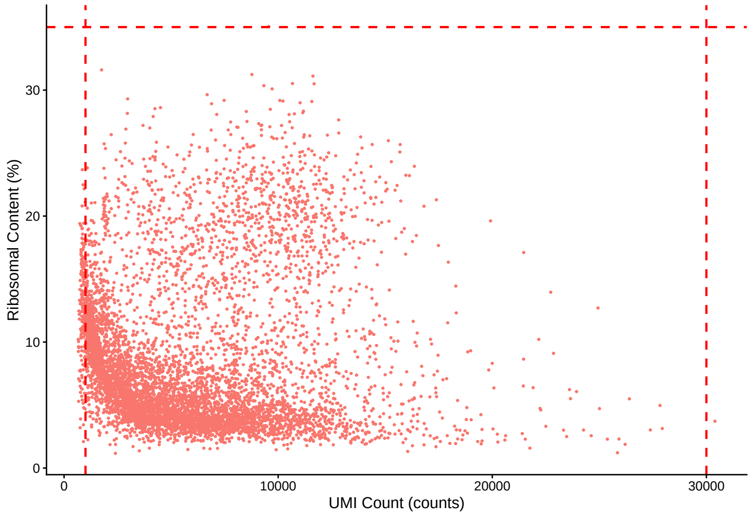
Ribosomal Content (%) vs UMI Count r = 0.03 – control
