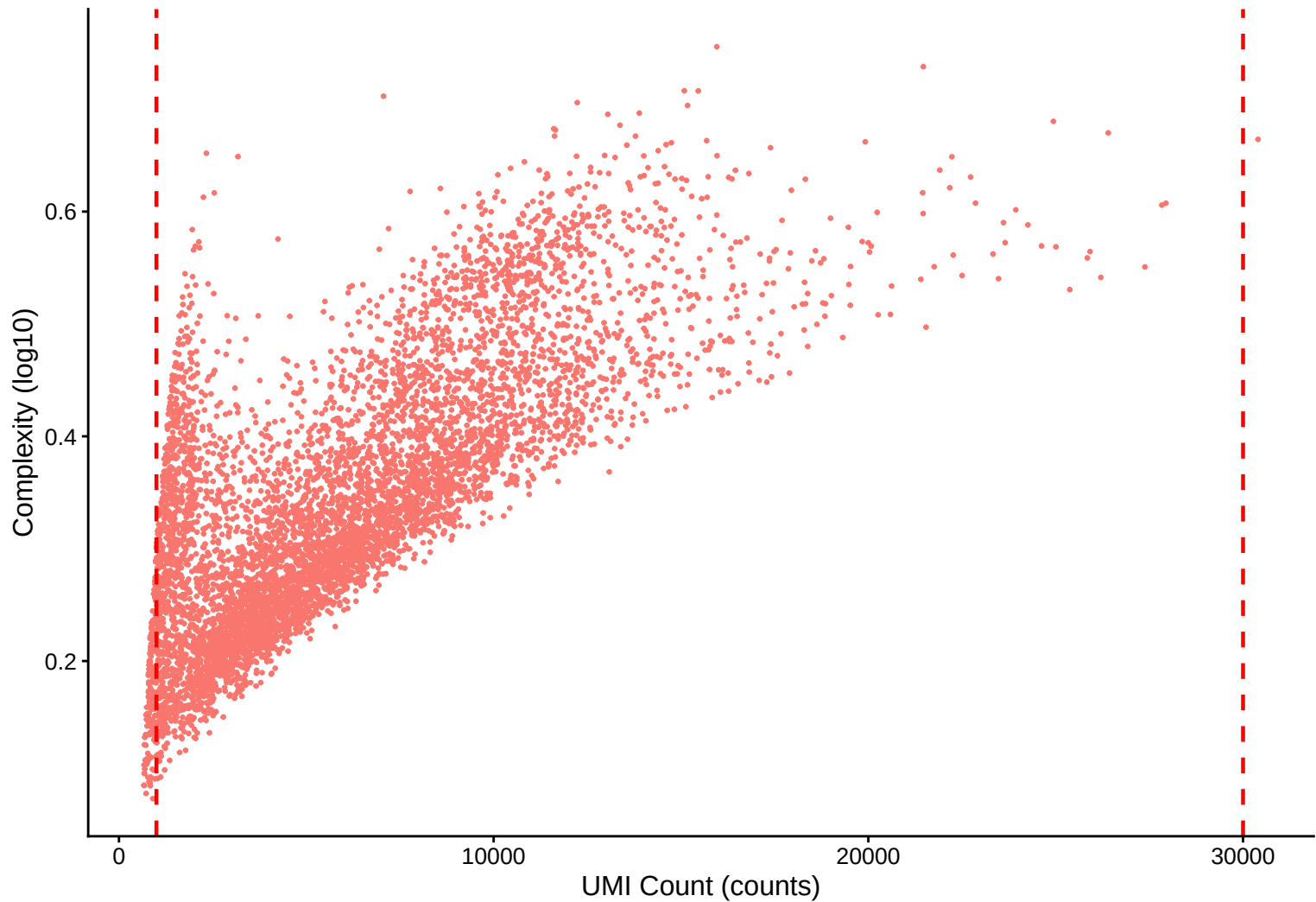
Complexity (log10) vs UMI Count r = 0.755 – control
