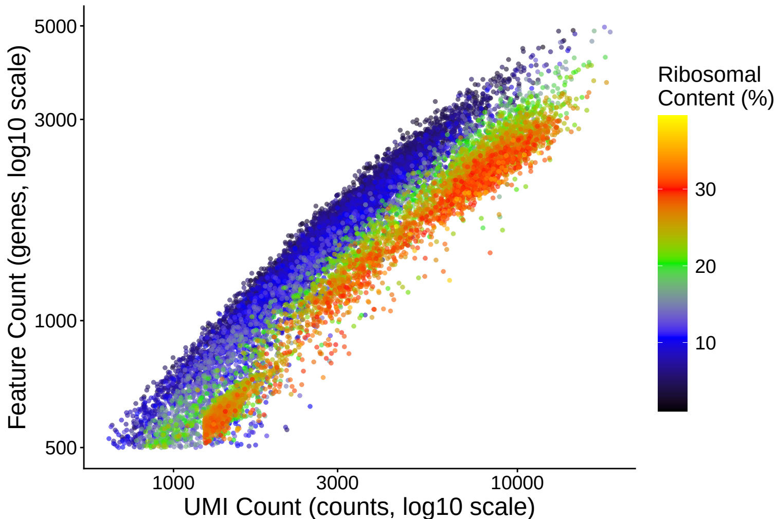
Feature vs UMI Count colored by Ribosomal Content r = 0.886 - 3h
