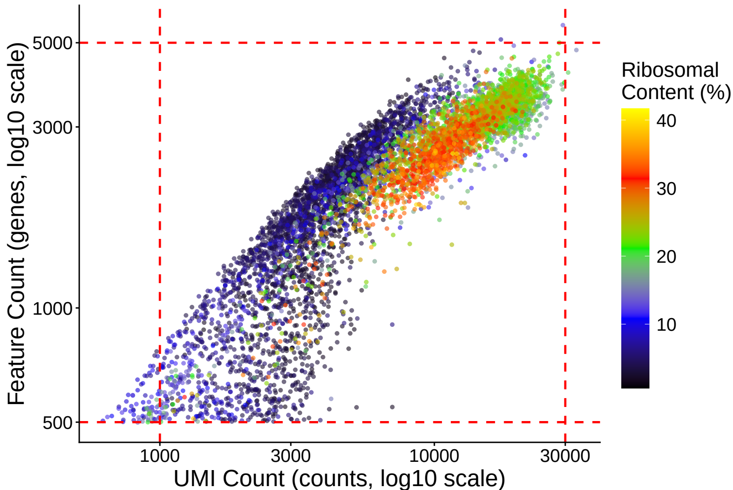
Feature vs UMI Count colored by Ribosomal Content r = 0.854 - 33\text{dpa}
