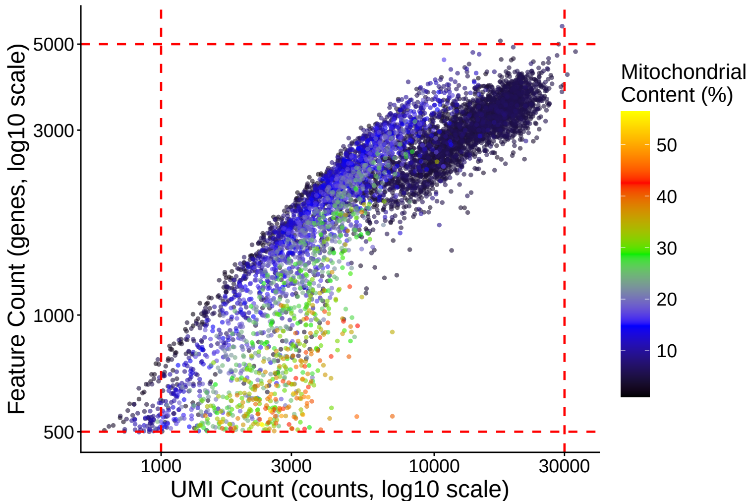
Feature vs UMI Count colored by Mitochondrial Content r = 0.854 - 33\text{dpa}
