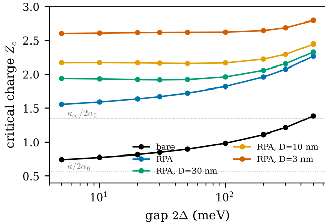
(b) j = 1/2 level reaches E = -\Delta
