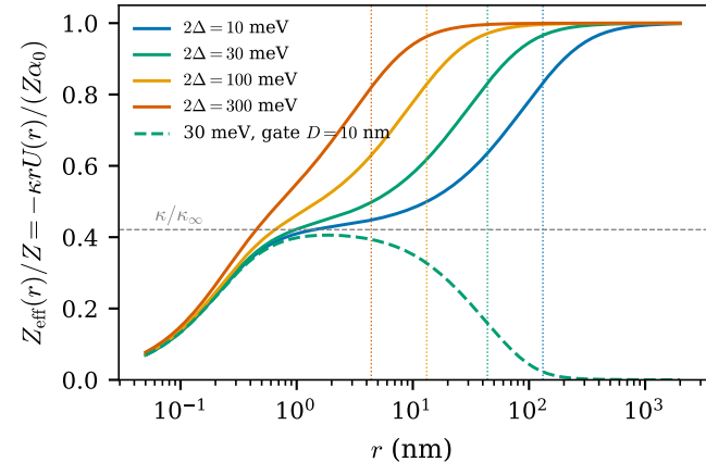
(a) Dirac-sea screening (dotted: \lambda_C = \hbar v / \Delta )
