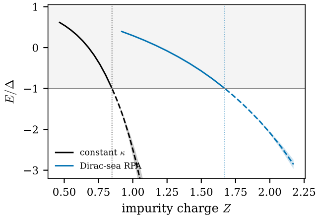
(a) 2\Delta = 30 meV: bound level (solid), resonance (dashed, band \pm\Gamma/2 )
