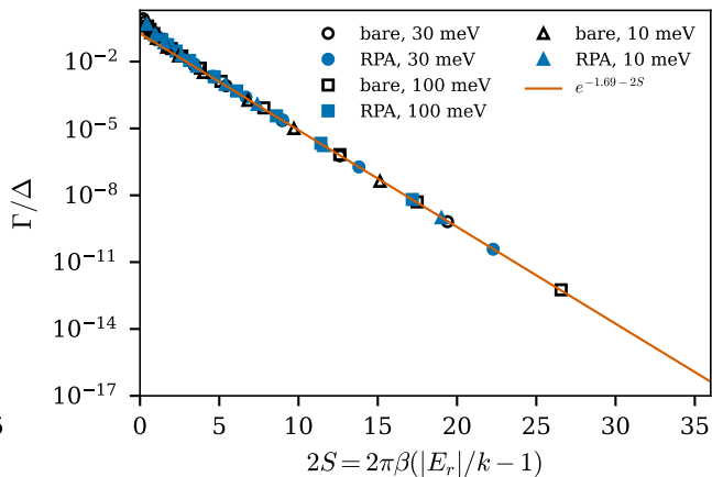
(b) Gamow law for the resonance width
