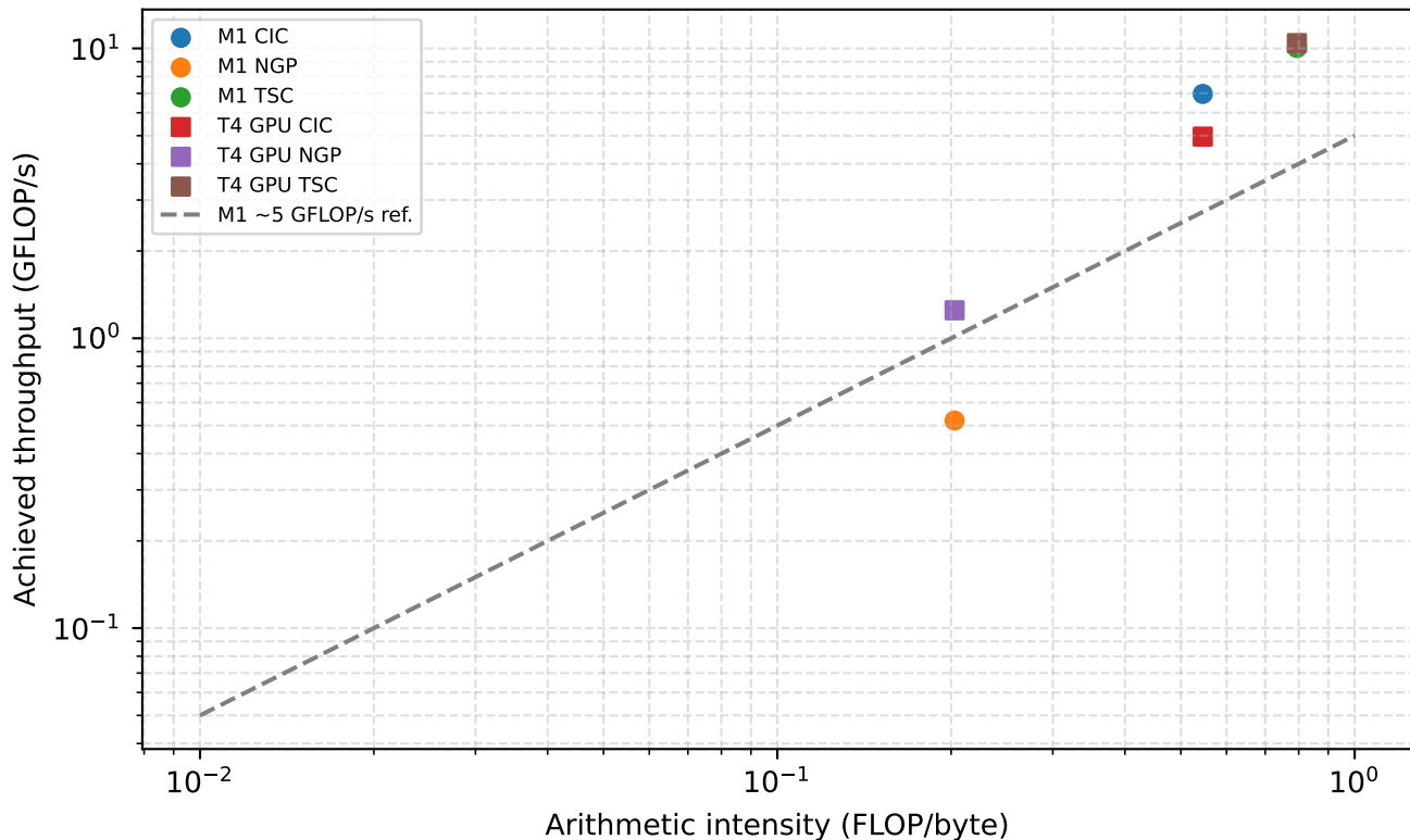
Roofline-style deposition performance (1e5, 128x128)
