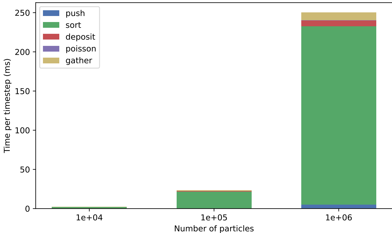
Full PIC timestep breakdown (CIC, SoA, sorted, 128x128)
