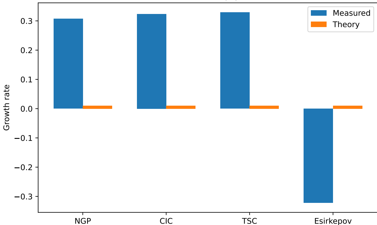
Two-stream instability growth rate
