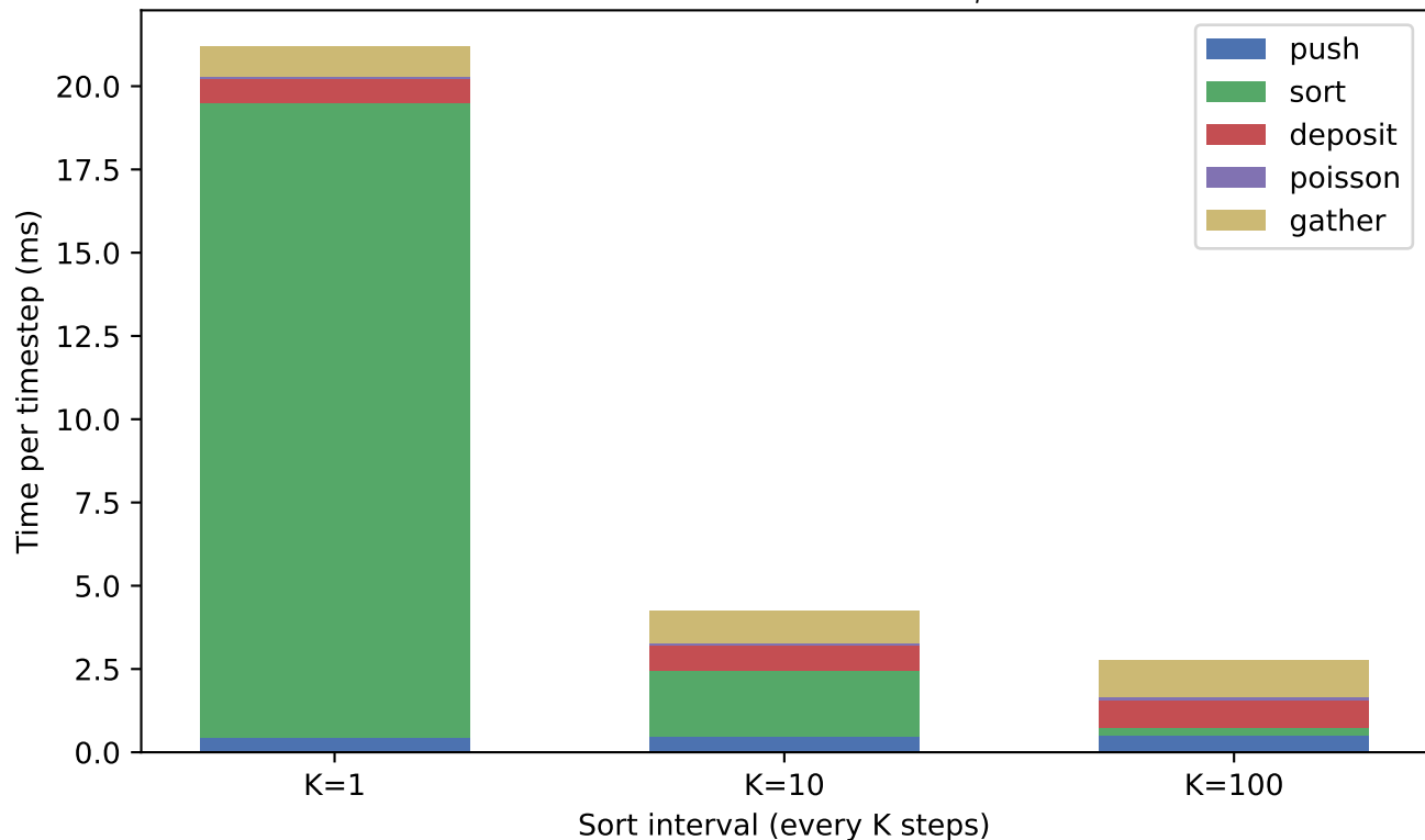
Amortized sort: CIC full timestep ( N_p = 10^5, 128^2 )
