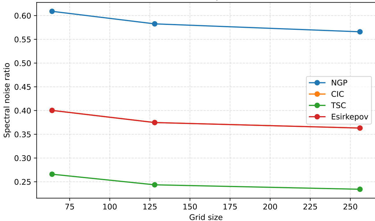
Spectral noise vs grid ( N_p = 10^5 , SoA sorted)
