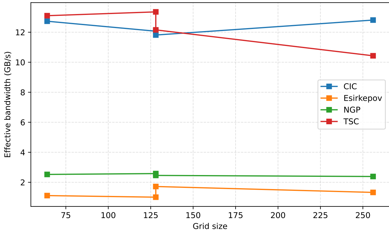
Memory bandwidth vs grid resolution (1e5 particles)
