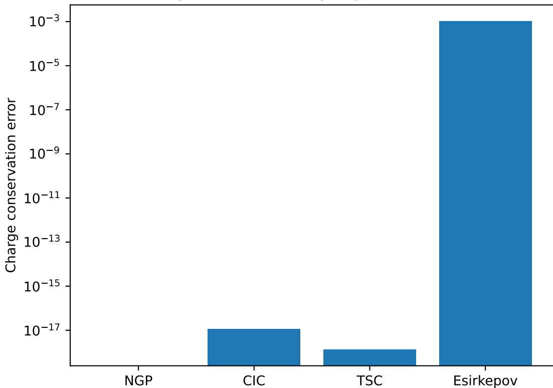
Charge conservation by deposition scheme
