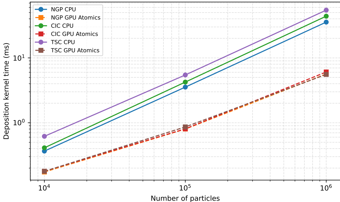
CPU vs GPU atomic deposition (128x128, SoA)
