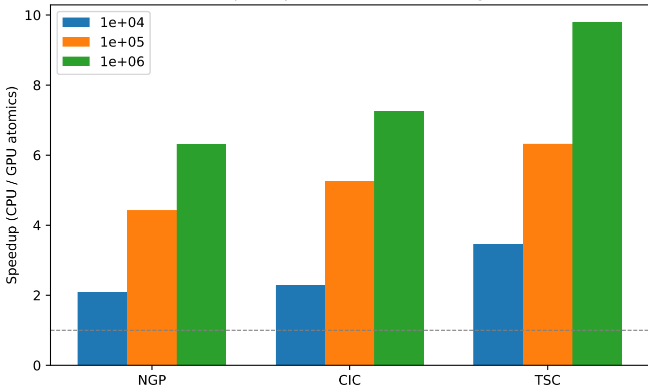
GPU speedup on Tesla T4 (128x128 grid)
