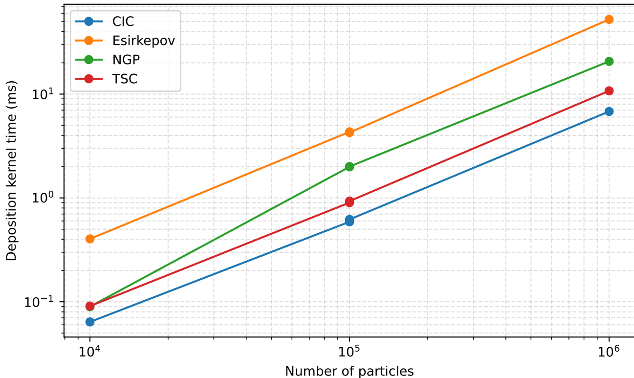
Deposition runtime vs particle count (128x128, SoA, sorted)
